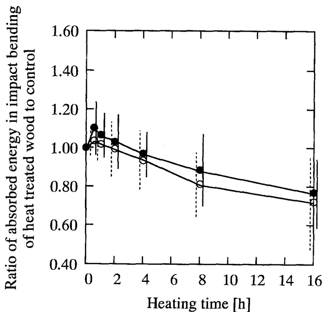
Fig. 14. Changes in absorbed energy in impact bending. Values are the average of the W_{ib}/W_{ibc} for each group, W_{ib} , absorbed energy in impact bending of heat-treated wood; W_{ibc} , absorbed energy in impact bending of control. Refer to Fig. 7 for explanation of symbols
