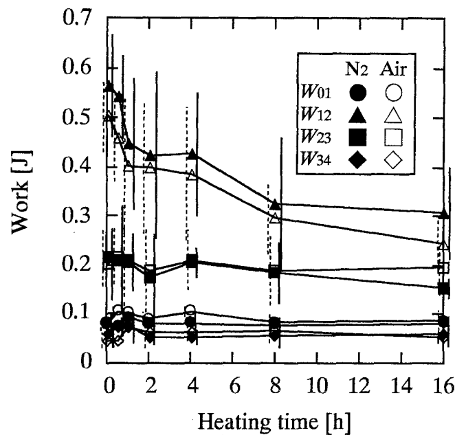
Fig. 13. Changes in work. Values are the average in each group. Filled circles , W_{01} of the specimens heat-treated in N_2 gas; filled triangles , W_{12} of the specimens heat-treated in N_2 gas; filled squares , W_{23} of the specimens heat-treated in N_2 gas; filled diamonds , W_{34} of the specimens heat-treated in N_2 gas; open circles , W_{01} of the specimens heat-treated in air; open triangles , W_{12} of the specimens heat-treated in air; open squares , W_{23} of the specimens heat-treated in air; open diamonds , W_{34} of the specimens heat-treated in air. Solid lines at the right of the filled symbols and dashed lines at the left of the open symbols are the standard deviation
