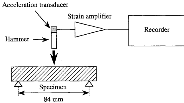
Fig. 3. Impact bending tester
