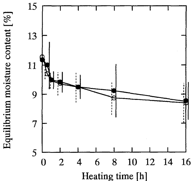
Fig. 9. Changes in equilibrium moisture content after heat treatment and immersion in water. Refer to Fig. 7 for explanation of symbols
