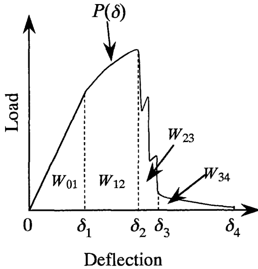
Fig. 2. Load-deflection curve
