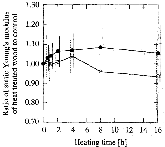
Fig. 10. Changes in static Young's modulus due to heat treatment. Values are the average of E/E_c in each group. E , static Young's modulus of heat-treated wood; E_c , static Young's modulus of control. Refer to Fig. 7 for explanation of symbols
