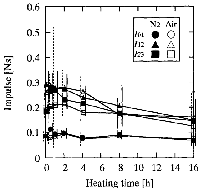
Fig. 15. Changes in impulse. Filled circles, I_{01} of the specimens heat-treated in N_2 gas; filled triangles, I_{12} of the specimens heat-treated in N_2 gas; filled squares, I_{23} of the specimens heat-treated in N_2 gas; open circles, I_{01} of the specimens heat-treated in air; open triangles, I_{12} of the specimens heat-treated in air; open squares, I_{23} of the specimens heat-treated in air. Solid lines at the right of the filled symbols or dashed lines at the left of the open symbols are the standard deviation
