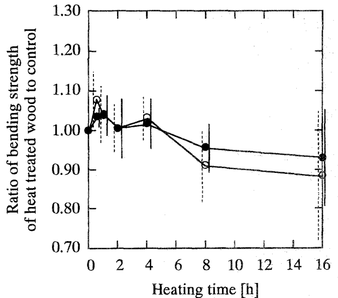
Fig. 11. Changes in bending strength due to heat treatment. Values are the average of \sigma/\sigma_c in each group. \sigma , bending strength of heat-treated wood; \sigma_c , bending strength of control. Refer to Fig. 7 for explanation of symbols
