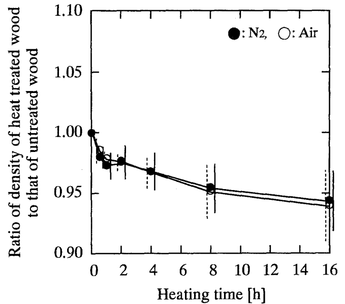
Fig. 7. Changes in density caused by heat treatment. The same specimens were used before and after treatment. Filled circles , specimens heat treated in N_2 gas; open circles , specimens heat treated in air. Solid lines at the right side of the filled circles and dashed lines at the left side of the open circles are the standard deviation
