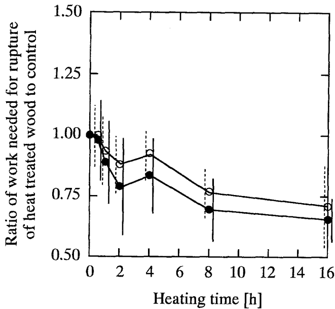
Fig. 12. Changes in work needed for rupture due to heat treatment. Values are the average of W_{04}/W_{04c} in each group. W_{04} , work needed for rupture of heat-treated wood; W_{04c} , work needed for rupture of control. Refer to Fig. 7 for explanation of symbols
