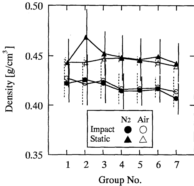
Fig. 5. Variation of density before heat treatment. Values are the average of each group. Filled circles , specimens heat-treated in N_2 gas for the impact bending test; open circles , specimens heat-treated in air for the impact bending test; filled triangles , specimens heat-treated in N_2 gas for the static bending test; open triangles , specimens heat-treated in air for the static bending test. Solid lines at the right side of the filled symbols or dashed lines at the left side of the open symbols are the standard deviation
