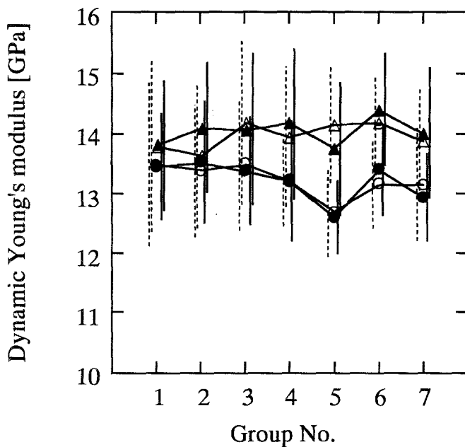
Fig. 6. Variation of dynamic Young's modulus before the heat treatment. Refer to Fig. 5 for explanation of symbols
