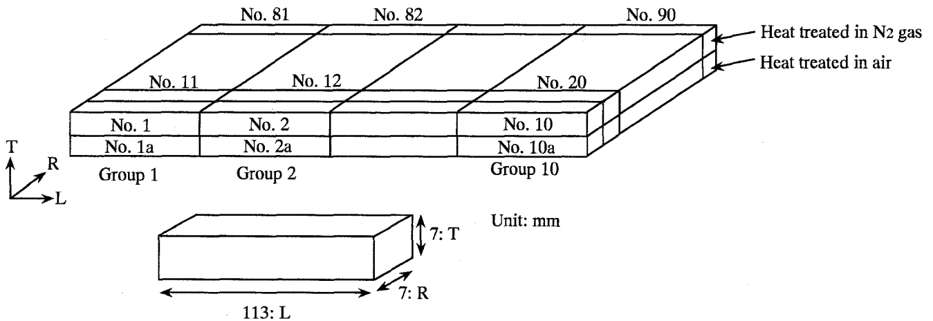
Fig. 1. Preparation of specimens
