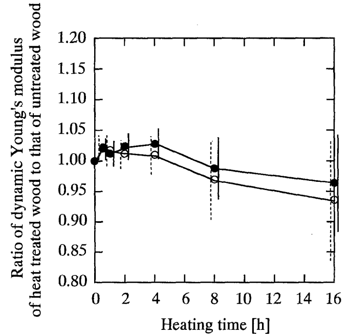
Fig. 8. Changes in dynamic Young's modulus caused by the heat treatment. Refer to Fig. 7 for explanation of symbols
