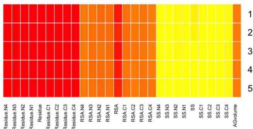
Figure 2. A heat map of each feature's impact on the 5 models generated from the 5-fold cross validation. Ranging from yellow to red, where yellow is low impact and red high impact. Each row specifies one cross-fold RF model and the columns specify the feature. The '.Nx' and '.Cx' suffix specifies positions relative to the investigated residue towards N and C-terminals, respectively.
