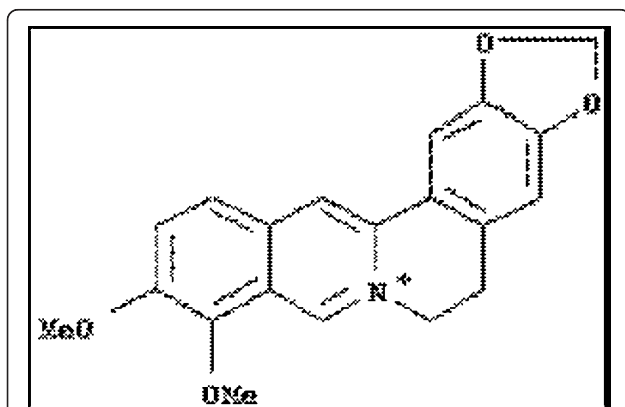
Chemical structure of berberine
