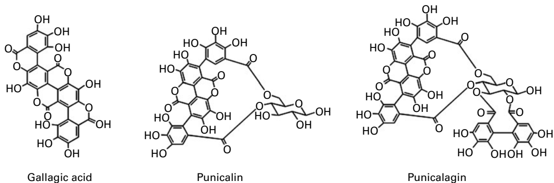
Fig. 6. Pomegranates contain gallagic acid and the ellagitannins punicalin and punicalagin.
