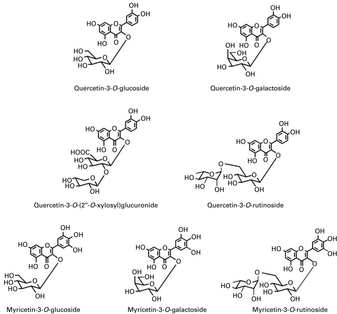
Fig. 3. Flavonols identified in berries.
