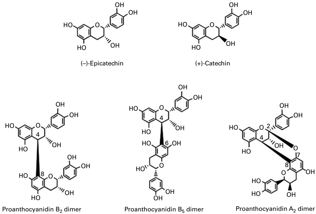
Fig. 4. Flavan-3-ol monomers and procyanidins identified in berries.
