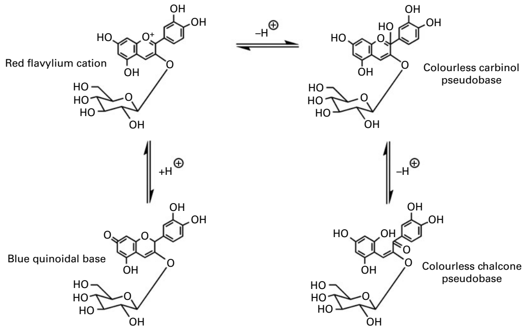
Fig. 9. Effect of pH on the structure of anthocyanins.
