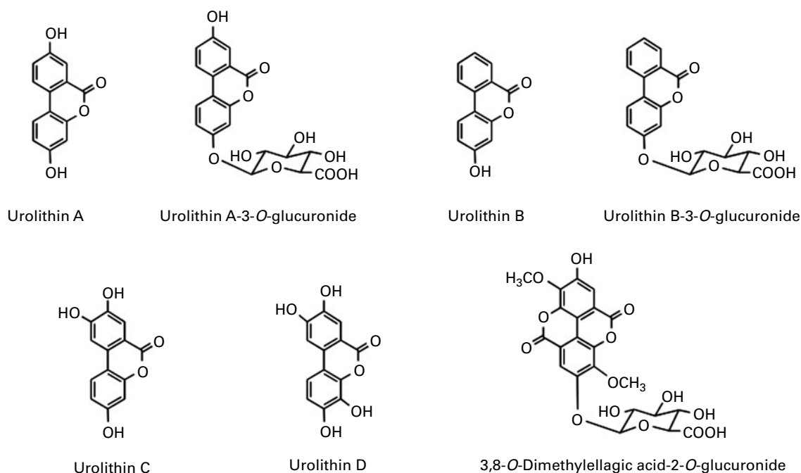
Fig. 11. Structures of urolithins and related compounds.
