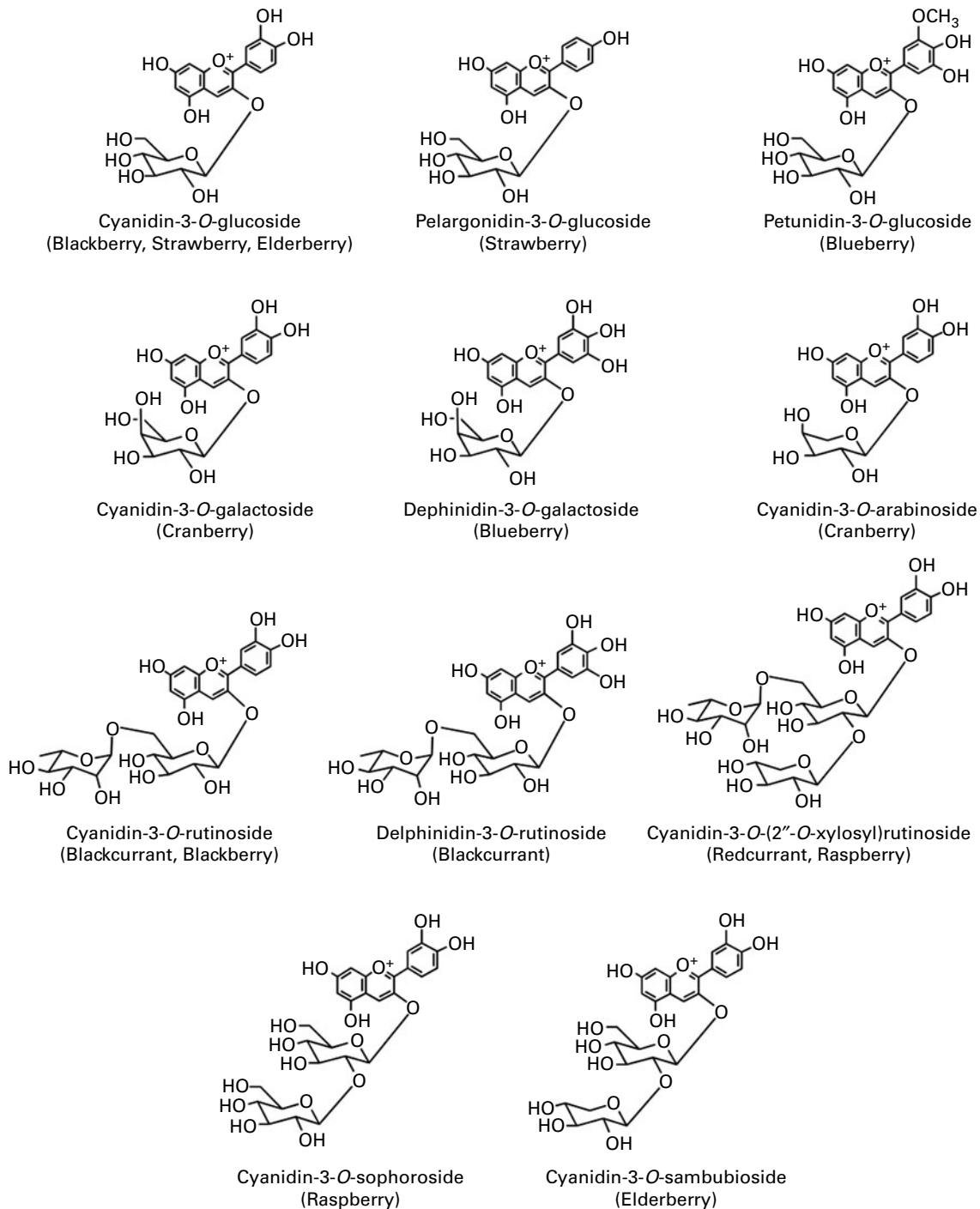
Fig. 2. Major anthocyanins in berries.
