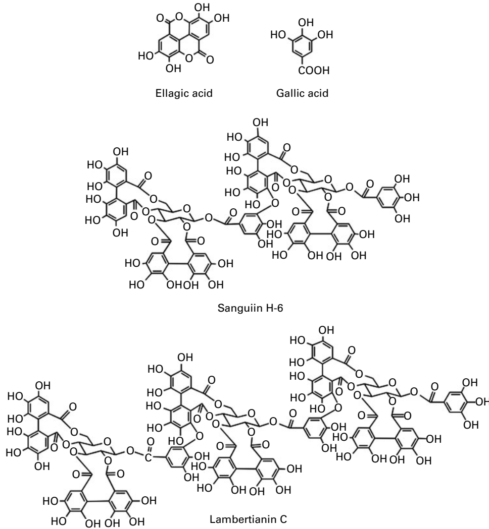
Fig. 5. Gallic acid, ellagic acid and the raspberry ellagitannins sanguin H-6 and lambertianin C.
