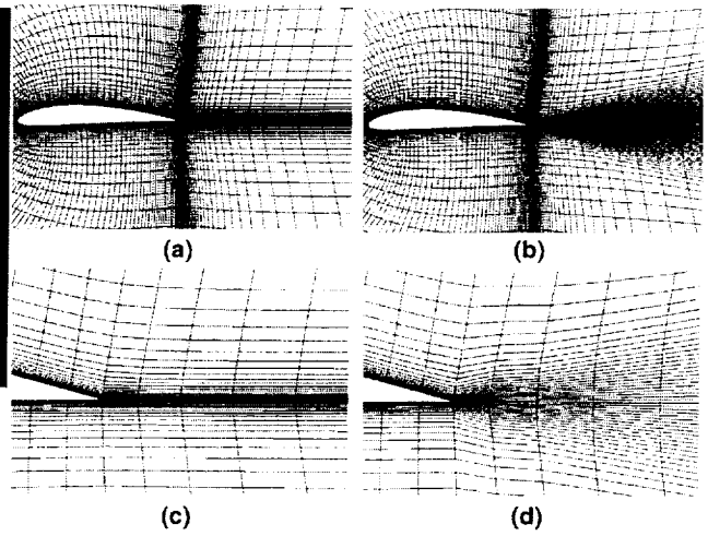
Fig. 22 Airfoil wake region. (a) Before smoothing (far view). (b) After smoothing (far view). (c) Before smoothing (close-up). (d) After smoothing (close-up).
