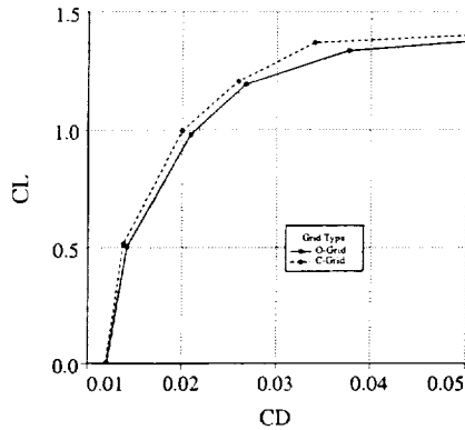
Fig. 21 Drag polars for a NACA 0015 airfoil using an O-grid (solid) and C-grid (dashed).
