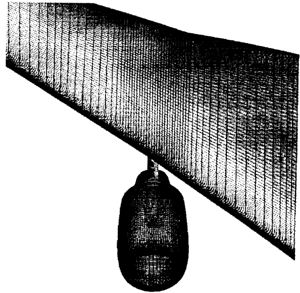
Fig. 16 Wing surface grid is refined near pylon attachment region to provide proper communication with pylon grids.
