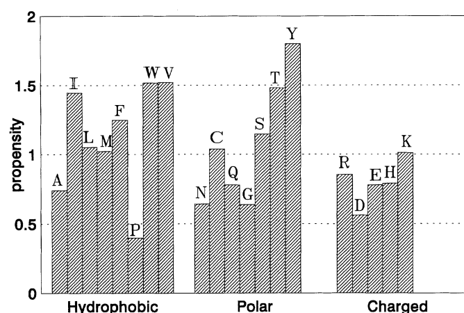
Fig. 9. Amino acid distribution in the strand segments of β-hairpins (see text for the definition of propensity value).
