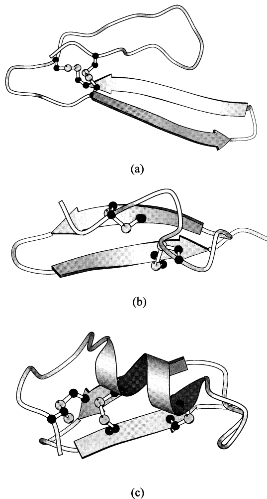
Fig. 12. Examples showing non-covalently linked Cys–Cys facing pairs in the strands. (a) Erabutoxin (3EBX 1–41), (b) E-Selectin (1ESL 120–146) and (c) scorpion neurotoxin (2SN3 15–50). The ribbon diagrams were prepared using the program MOLSCRIPT (Kraulis, 1991).
