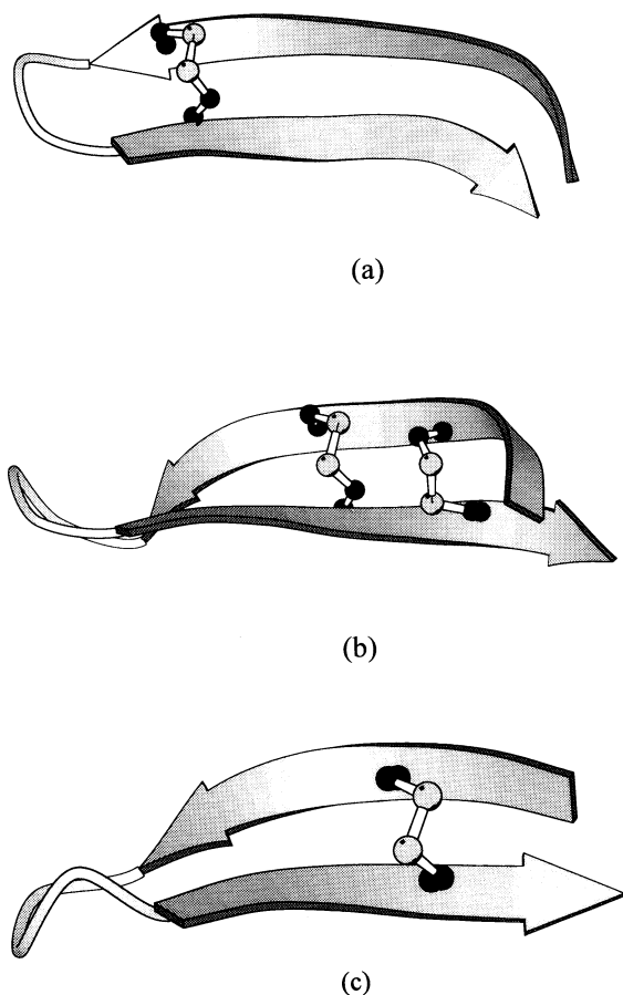
Fig. 11. Examples showing Cys–Cys facing pairs in the strand segments which are covalently linked. (a) Neuraminidase (INSC A 114–132), (b) neuraminidase (INSC A 273–292) and (c) diphtheria toxin (1DDT 459–473). The ribbon diagrams were prepared using the program MOLSCRIPT (Kraulis, 1991).
