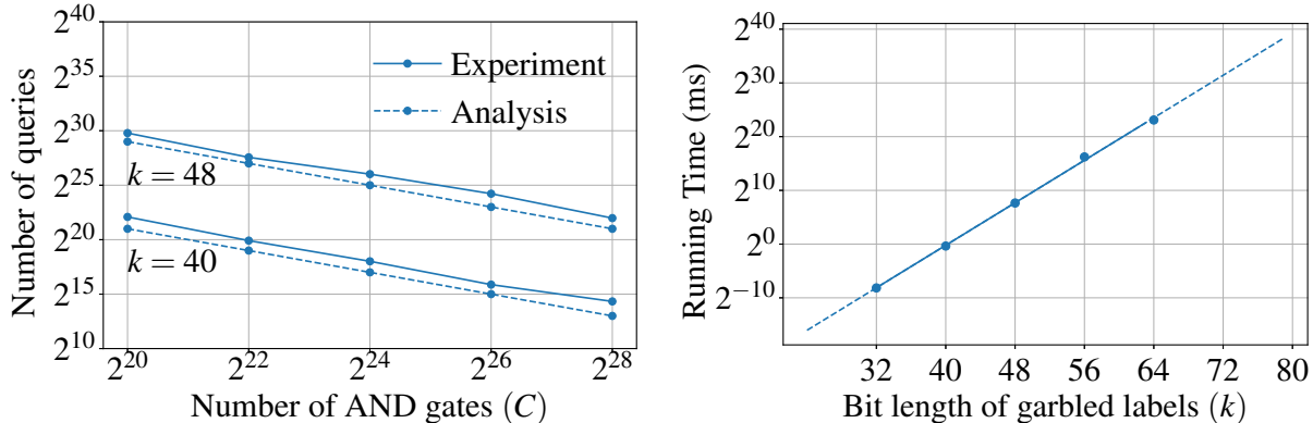
(a) Number of \pi -queries for the attack to succeed, on a log/log scale. (b) The running time of our attack with C = 2^{30} and different values of k .
