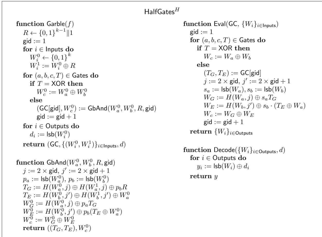
Figure 1: The half-gates scheme based on a hash function H .
