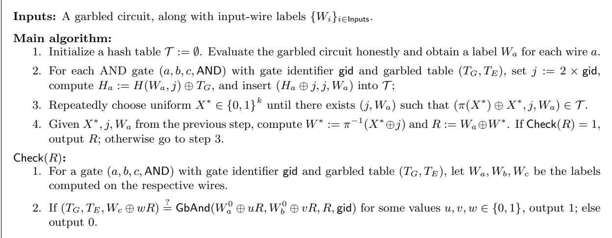
Figure 4: Attack on the \text{TMMO}^\pi -based implementation of the half-gates scheme.
