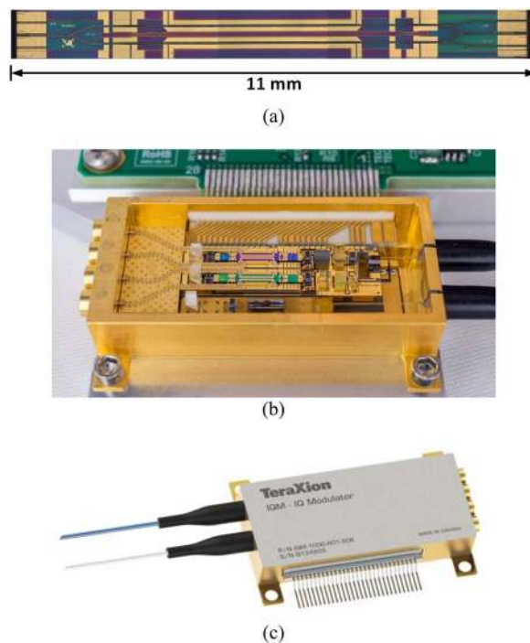
Fig. 9. InP modulator: (a) InP chip, (b) open, and (c) closed package for InP dual-polarization I/Q modulator, respectively.
