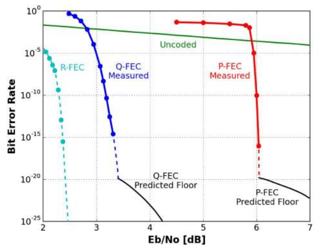
Fig. 20. Performance of various generations of FECs.
