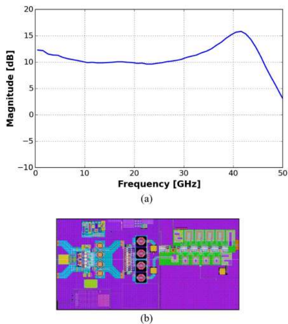
Fig. 7. VGA: (a) measured frequency response (10 dB gain shown) and (b) chip layout.
