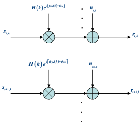
Fig. 3. (Color online) Equivalent OFDM channel model. \phi_{CD}(k) denotes the phase distortion of the k th subcarrier due to chromatic dispersion.
