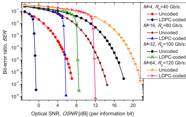
Fig. 5. (Color online) BER performance of the proposed polarization multiplexed coded-OFDM scheme, for DGD of 1200 ps and the worst-case scenario ( \theta = \pi/2 , \varepsilon = 0 ). R_D denotes the aggregate data rate.
