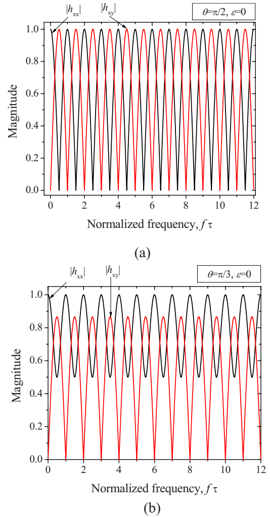
Fig. 1. (Color online) Magnitude response of h_{xx} and h_{xy} Jones matrix coefficients against the normalized frequency for (a) \theta = \pi/2 and \varepsilon = 0 , and (b) \theta = \pi/3 and \varepsilon = 0 .
