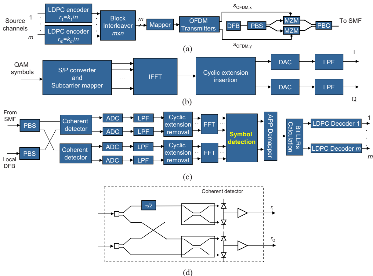
Fig. 2. (Color online) The architecture of the polarization-multiplexed LDPC-coded OFDM scheme: (a) transmitter architecture, (b) OFDM transmitter architecture ( x - or y -polarization), (c) receiver architecture, and (d) balanced coherent detector configuration. DFB, distributed feedback laser; PBS(C), polarization beam splitter (combiner); MZM, dual-drive Mach-Zehnder modulator; APP, a posteriori probability; LLRs, log-likelihood ratios.
