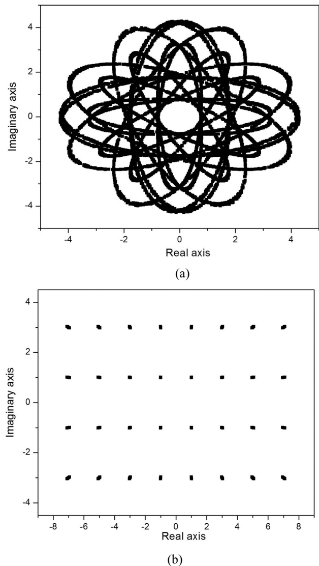
Fig. 4. The constellation diagrams for M=32 QAM (the aggregate data rate is 100 Gb/s) after 1200 ps of DGD observing the worst-case scenario ( \theta = \pi/2, \varepsilon = 0 ) (a) before PMD compensation and (b) after PMD compensation.
