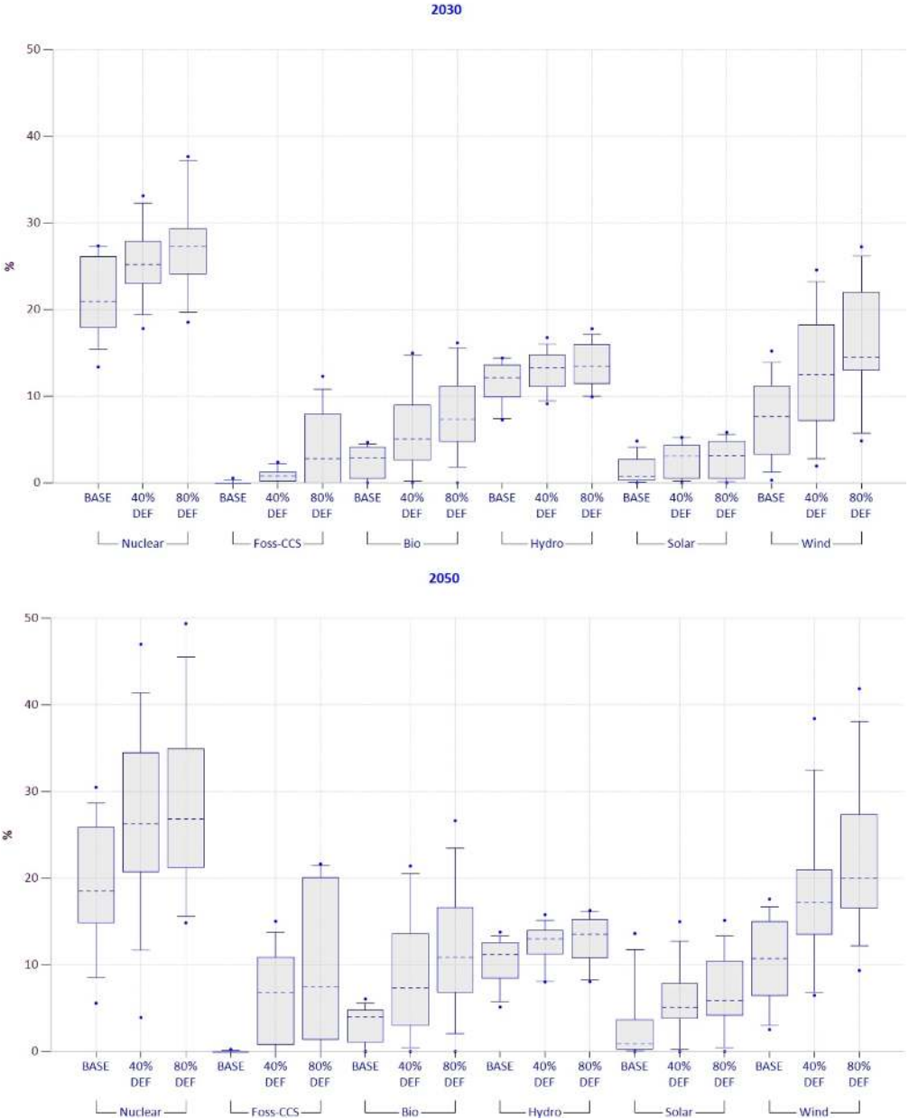
Figure 5. Percentage share of low carbon technologies in electricity mix for 2030 (upper panel) and 2050 (lower panel). The dotted line is the median, the box contains the 50% interval, the whiskers mark the 90% interval, and the dots mark the extreme values.
