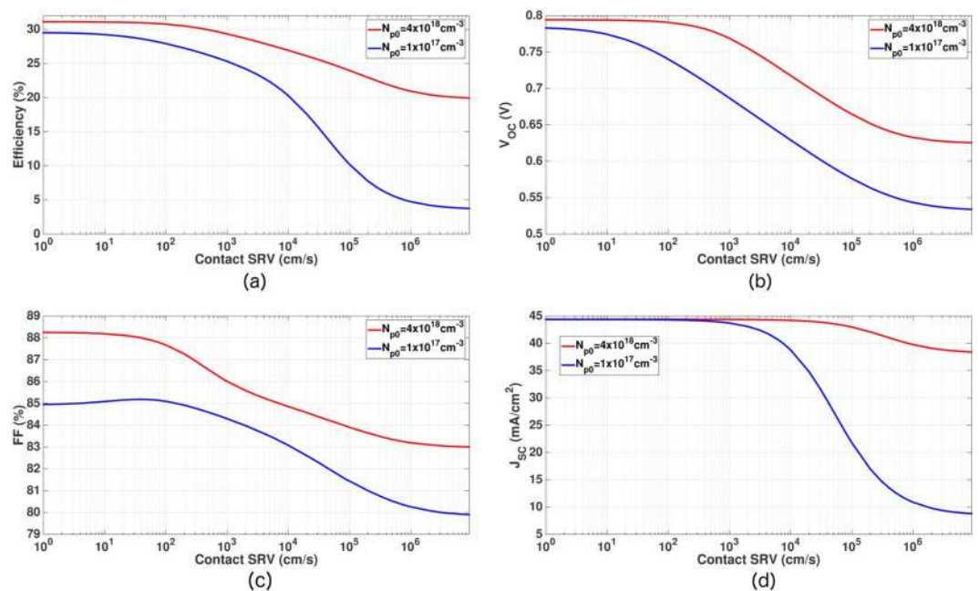
Figure 12. Effect of contact SRV on the performance parameters of the proposed inverted pyramid PhC IBC cell with H = 15\ \mu\text{m} and \tau_{SRH} = 10\ \text{ms} (other design parameters are specified in Table 4). The red curve corresponds to optimum FSF and BSF doping, showing a more gradual drop in the cell efficiency as contact SRV increases. In contrast, a rapid degradation in cell efficiency (blue curve) when FSF/BSF dopings are improperly chosen.
