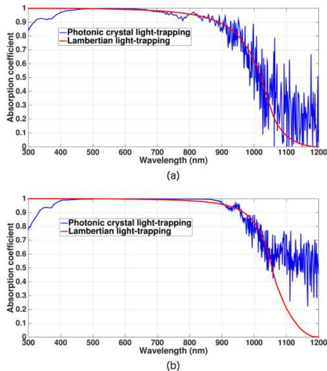
Figure 4. Absorption spectra for (a) 5\ \mu\text{m} and (b) 15\ \mu\text{m} -thick inverted pyramid photonic crystal IBC solar cell over the 300–1200 nm wavelength range (blue curves). The 1100–1200 nm absorption is modeled following the details illustrated in the “Methods” section. Red curves correspond to the absorption spectra of the hypothetical Lambertian cells. In contrast to Lambertian cells and planar cells, high solar energy absorption in the 950–1200 nm spectral range due to multiple resonant absorption peaks is a signature of photonic crystal light-trapping.
