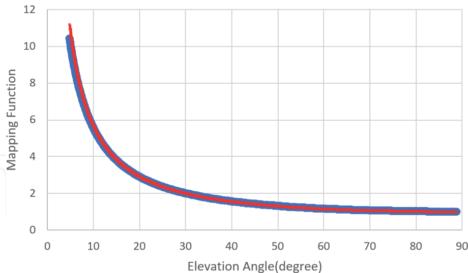
Mapping function versus elevation BJFS (Beijing)
