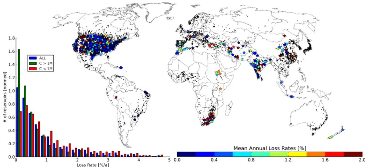
Figure 1. Location of 1215 case studies with observed reservoir sedimentation rates (colored stars, see scale bar), and location of 6399 GReservoirs (small black dots). Inset: histogram of 1215 observed annual reservoir capacity loss rates, as percentage of installed capacity, grouped by capacity larger than 1 million \text{m}^3 and smaller than 1 million \text{m}^3 .
