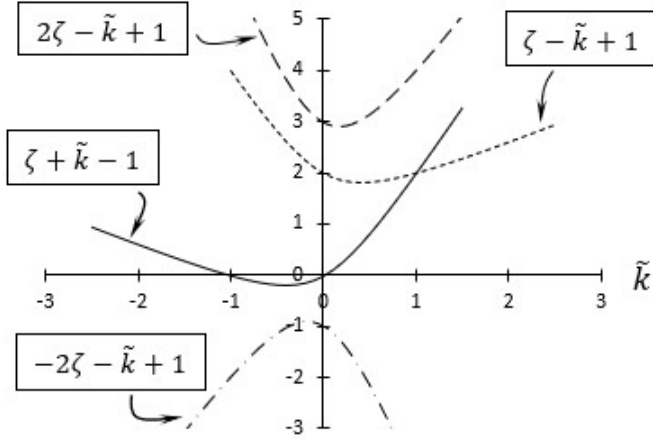
Figure 7: Various combinations of \tilde{k} and \zeta , to be used in this paper, as functions of \tilde{k} .
