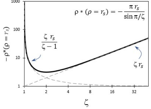
Figure 11: \rho^*(\rho = r_s) as function of \zeta ; both axes in log scale (with r_s = 1 ). The two asymptotes are \zeta/(\zeta - 1) (for \tilde{k} \rightarrow 0 ) and \zeta (for \tilde{k} \rightarrow \infty ). Note that \rho^*(\rho = r_s) = -\pi for \tilde{k} = 1 .
