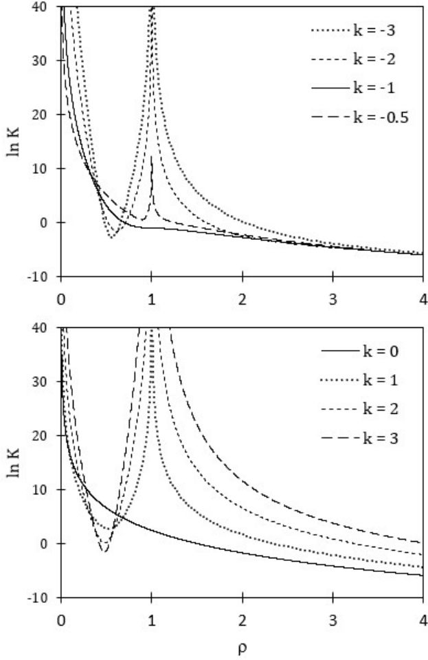
Figure 8: Logarithm of Kretschmann invariant as function of the new coordinate \rho , for various value of \tilde{k} . For clarity, we plot the curves in two panels. In all cases, r_s = 1 .
