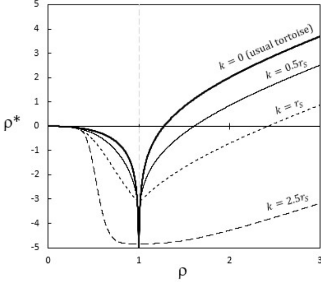
Figure 10: The \zeta -tortoise coordinate of Eq. (135) for various values of \tilde{k} (with r_s = 1 ).
