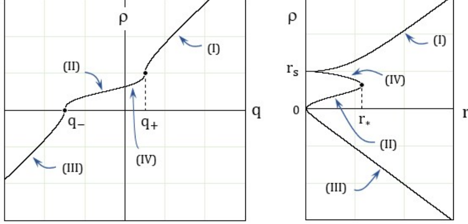
Figure 4: \rho as functions of q and r . Plots are for r_s = 1 , k = r_s .
