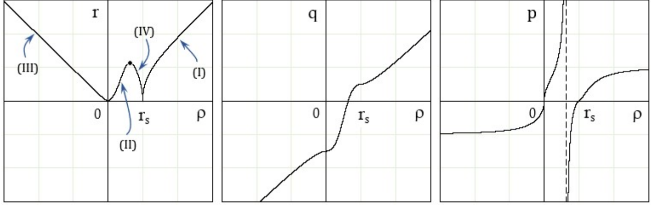
Figure 5: Various variables as functions of \rho . Plots are for r_s = 1 , k = r_s .
