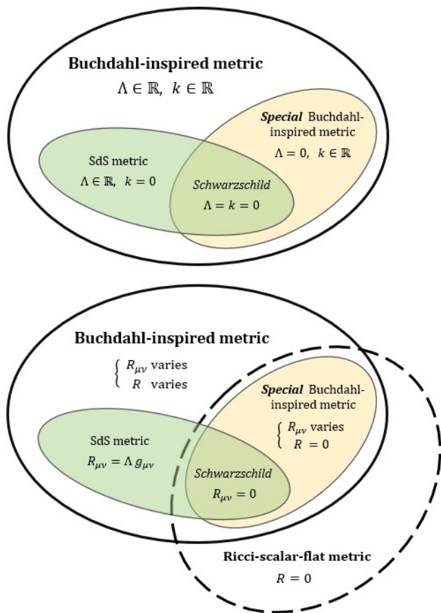
Figure 1: Upper panel: the Buchdahl-inspired metric family and its subsets. Lower panel: their relation with the Ricci-scalar-flat family. The special Buchdahl-inspired metric in the intersection is asymptotically flat, whereas the Buchdahl-inspired metric with \Lambda \neq 0 is asymptotically constant.
