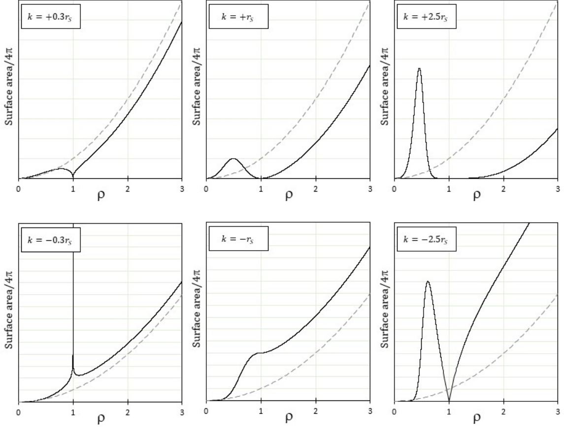
Figure 9: Surface area as function of the new coordinate \rho . Upper panels: \tilde{k} = 0.3, 1, 2.5 . Lower panels: \tilde{k} = -0.3, -1, -2.5 . The dash line in each panel is the trivial \tilde{k} = 0 benchmark, A = 4\pi\rho^2 .
