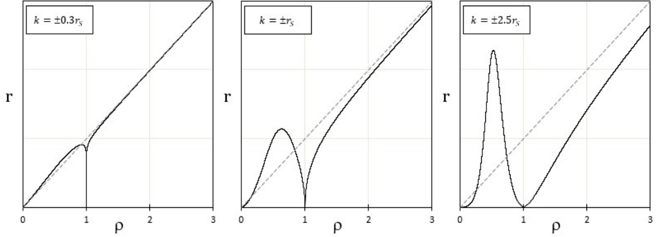
Figure 6: Areal coordinate r as function of the new coordinate \rho . For \tilde{k} = \pm 0.3, \pm 1, \pm 2.5 . In all plots, r_s = 1 .
