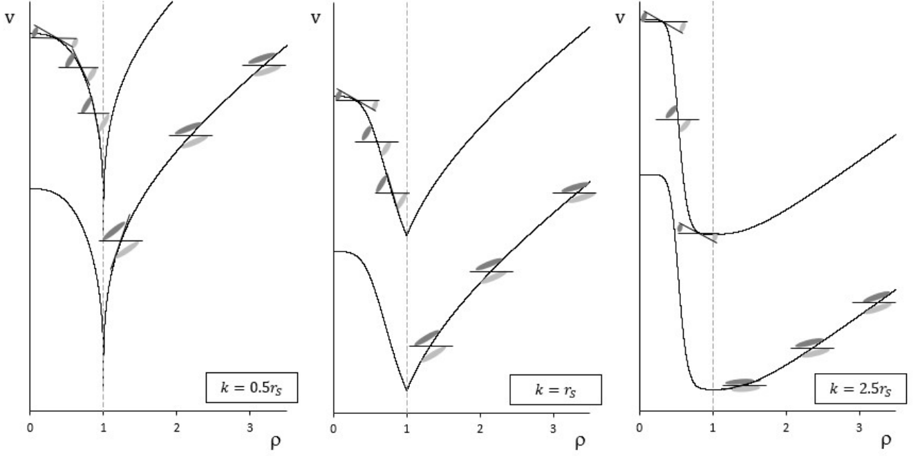
Figure 12: Light cones in the (\rho, v) plane (with r_s = 1 ), for \tilde{k} = 0.5, 1, 2.5 . We choose these values of \tilde{k} as representatives for the three cases discussed in the text.
