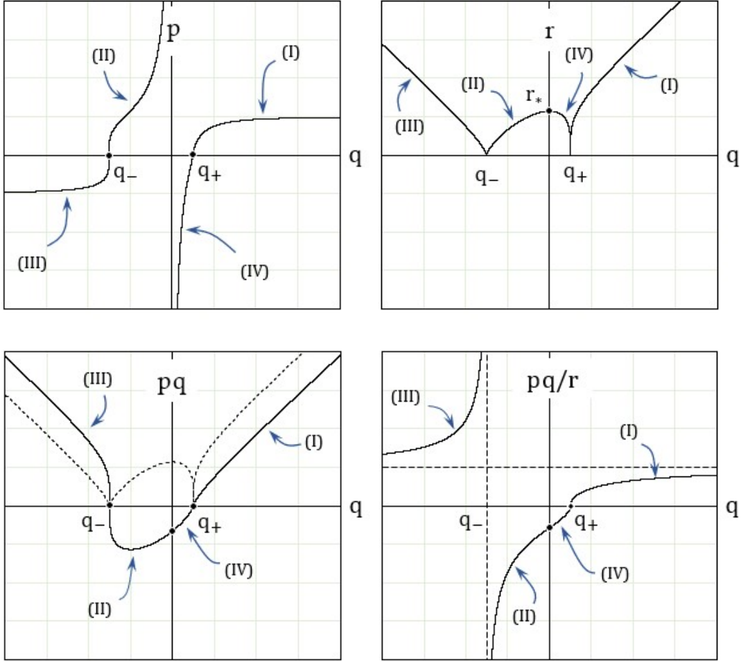
Figure 2: Plots of p , r , pq and pq/r as functions of q . Plots are for r_s = 1 , k = r_s . See Remark 4 for explanations.
