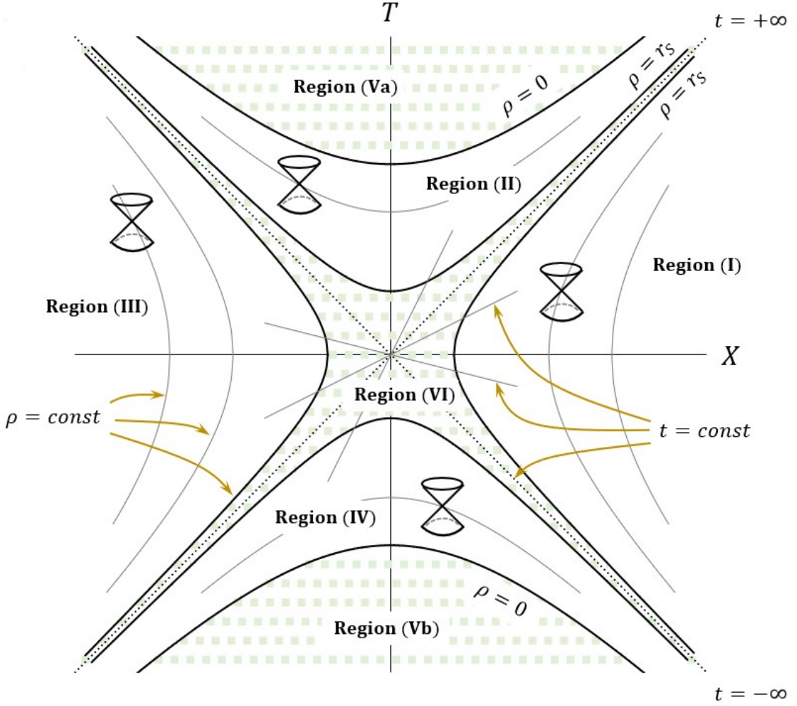
Figure 13: Kruskal-Szekeres diagram for \tilde{k} \neq 0 . The “gulf” shown as Region (VI) is a new feature. See text for explanations.
