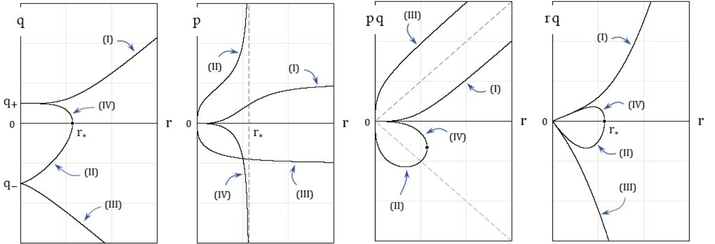
Figure 3: Plots of q , p , pq and rq as functions of r . Plots are for r_s = 1 , k = r_s . The leftmost panel reveals the multi-valuedness problem for q(r) .
