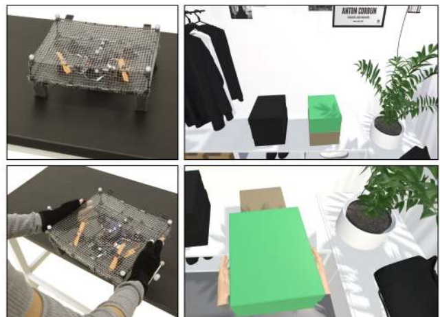
Figure 13: Dynamic positioning of passive haptics: quad landing on a table in the room to render a shoebox, and user picking up the shoebox.
