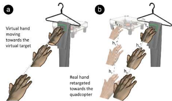
Figure 5: Visuo-haptic illusions are used to compensate for lack of control accuracy. (a) Quad is accurately positioned and no illusion is needed. (b) To correct for the position offset, as the virtual hand touches the virtual target, body warping is used to retarget the hand towards the quad.
