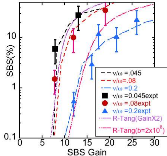
FIG. 1: The SBS reflectivity is shown as a function of the calculated gain for both experiments and pF3D simulations. The results for different \nu/\omega are denoted with different colors. The symbols with error bars represent the SBS measured at OMEGA in hohlraum experiments. The dashed lines are pF3D calculations of the level of backscatter. The purple and magenta dash-dotted curves are results from Eq. 3 with the gain multiplied by 2 and b = 1 \times 10^{-9} and with the nominal gain and b = 2 \times 10^{-8} .
