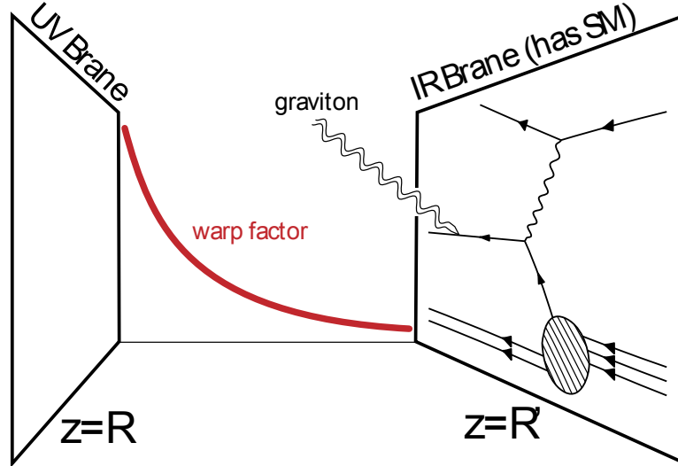
Fig. 5: Cartoon of the RS scenario with a brane-localized SM. The warp factor, (R/z)^2 , causes energy scales to be scaled down towards the IR brane.
