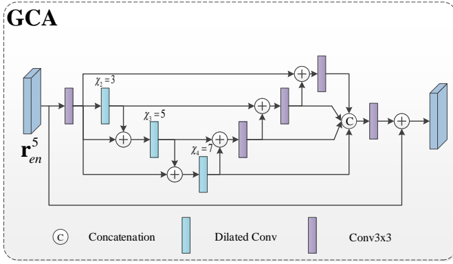
Fig. 4. Architecture of our proposed GCA module. First, some convolutional layers with different dilation rates are employed to extract multi-scale features. Then, some bottom-up and top-down pathways as well as some skip connections are employed to achieve the interactions among multi-scale features. Finally, the original information is added to the aggregated multi-scale features for obtaining the final output features.
