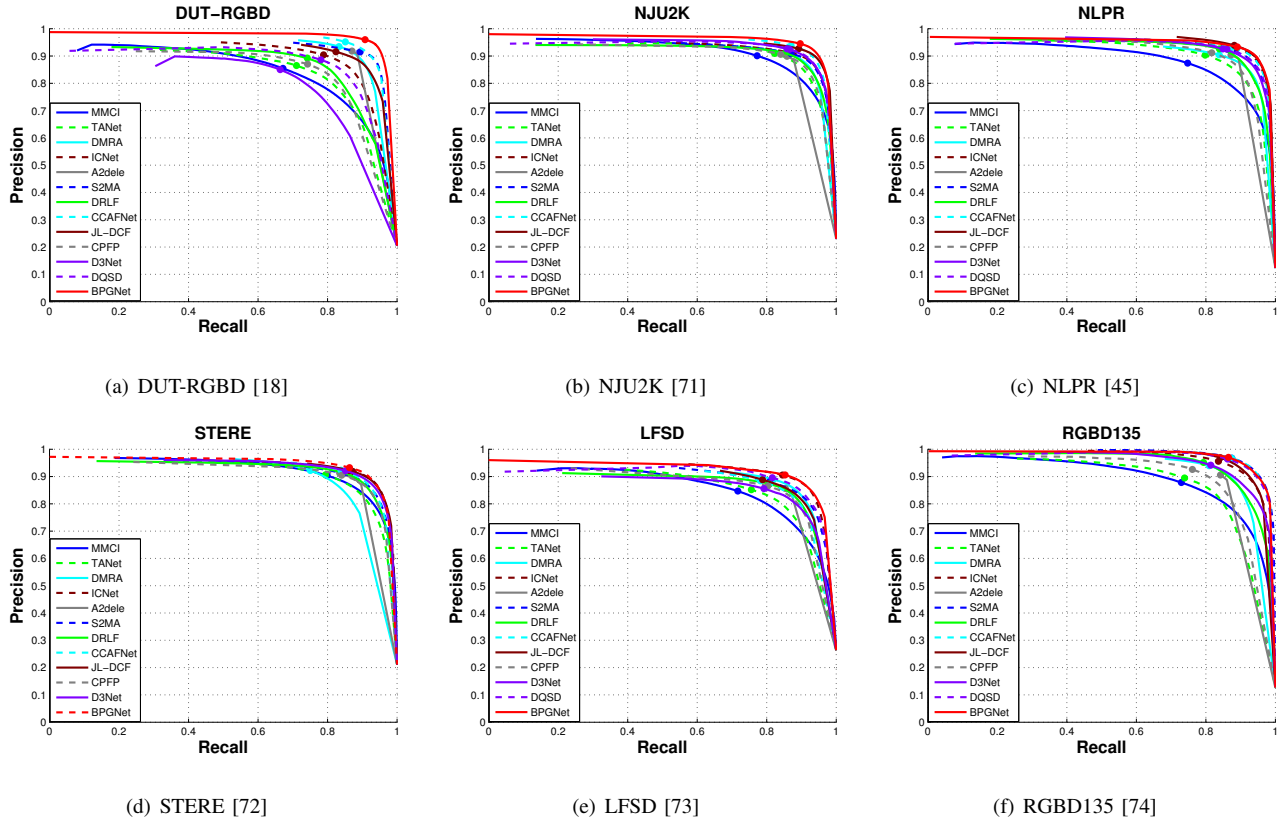
Fig. 8. Quantitative comparisons of our method with other methods on six challenging benchmark datasets.
