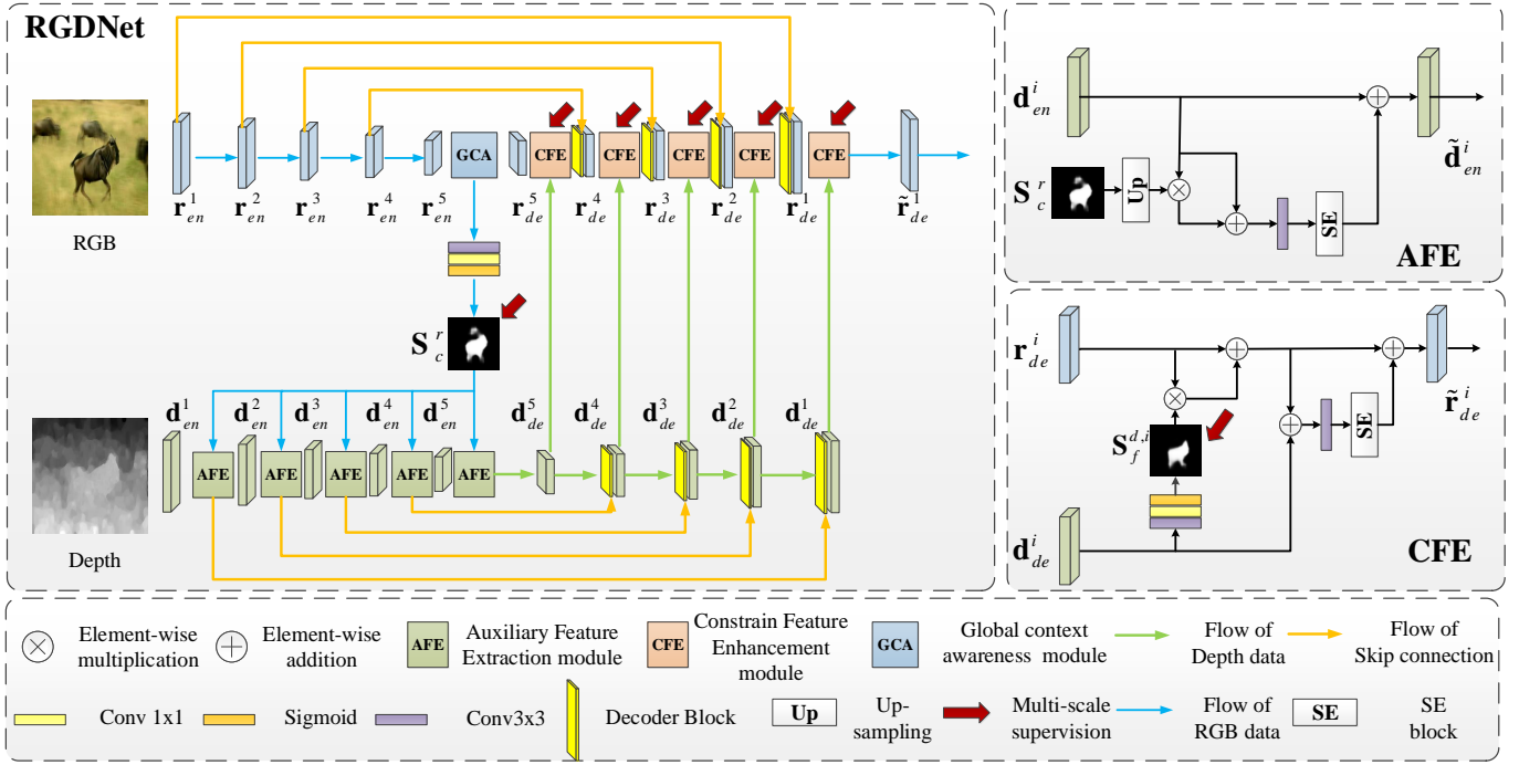
Fig. 3. Architecture of our proposed RGDNet, which contains three key stages: coarse saliency map generation, feature extraction and feature enhancement. First, GCA is used to capture global contextual information from the deepest level of encoded RGB features to obtain a coarse saliency map, which is fed into AFE as the guidance to help extract depth features. Finally, the extracted depth features are transferred to CFE for the enhancement of RGB features. For better visualization, we ignore the convolutional layer in the skip connection for compressing channels.
