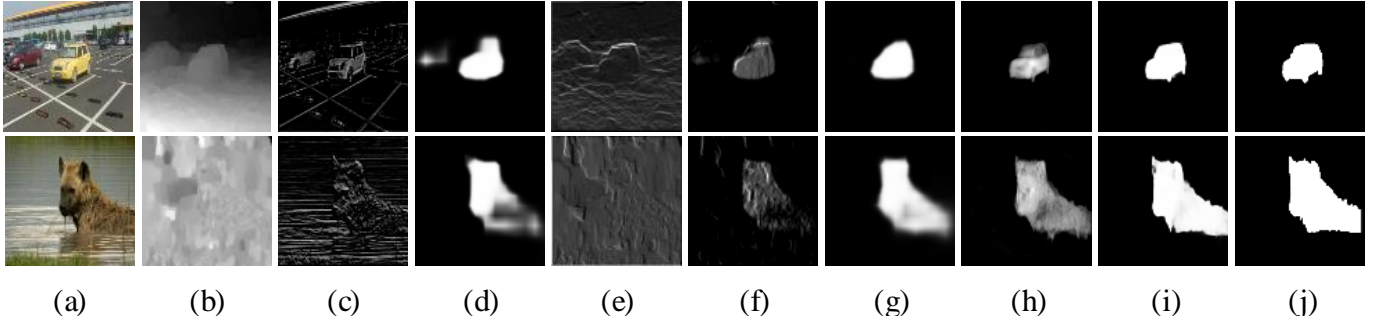
Fig. 5. Visual examples of some intermediate results from RGDNet. From left to right: (a) RGB images; (b) Depth images; (c) Original RGB features \mathbf{r}_{en}^1 ; (d) Coarse saliency maps \mathbf{S}_c^r ; (e) Original depth features \mathbf{d}_{en}^1 ; (f) Enhanced depth features \tilde{\mathbf{d}}_{en}^1 obtained by AFE; (g) Refined saliency maps \mathbf{S}_f^{d,5} ; (h) Enhanced RGB features \tilde{\mathbf{r}}_{de}^1 obtained by CFE; (i) Refined saliency maps \mathbf{S}_R^i deduced from (h); (j) GT.
