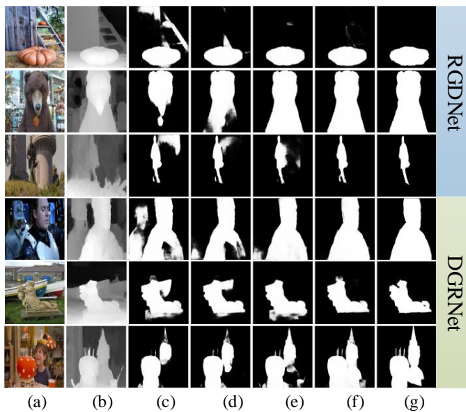
Fig. 9. Some visual comparisons on RGDNet and DGRNet. (a) RGB images; (b) Depth images; (c) B; (d) B+GCA; (e) B+GCA+AFE; (f) B+GCA+AFE+CFE; (g) GT. In the first three rows, some high-quality RGB images and relatively low-quality depth images are used to verify the effectiveness of each component on RGDNet. While, in the last three rows, some high-quality depth images and relatively low-quality RGB images are used to verify the effectiveness of each component on DGRNet.
