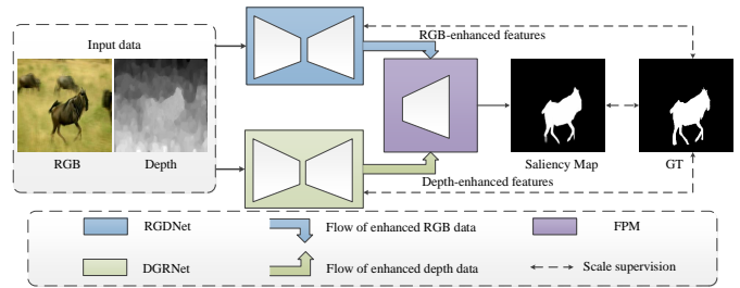
Fig. 2. Overall architecture of the proposed BPGNet, including three parts, i.e., RGDNet, DGRNet and FPM. RGDNet and DGRNet are used to achieve extract and enhance unimodal features, while FPM is used to combine the enhanced unimodal features for final saliency prediction.
