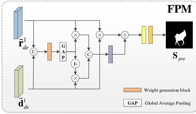
Fig. 6. Architecture of our proposed Fusion Prediction Module (FPM). First, we adopt the concatenation-convolution operation to learn the complementarity weights for different enhanced features. Secondly, we adopt multiplication operation to learn common information and strengthen the response of salient objects. Subsequently, the addition operation is used to obtain the final fused features. Finally, the fused features are mapped to a final saliency map through a 1 \times 1 convolutional layer.
