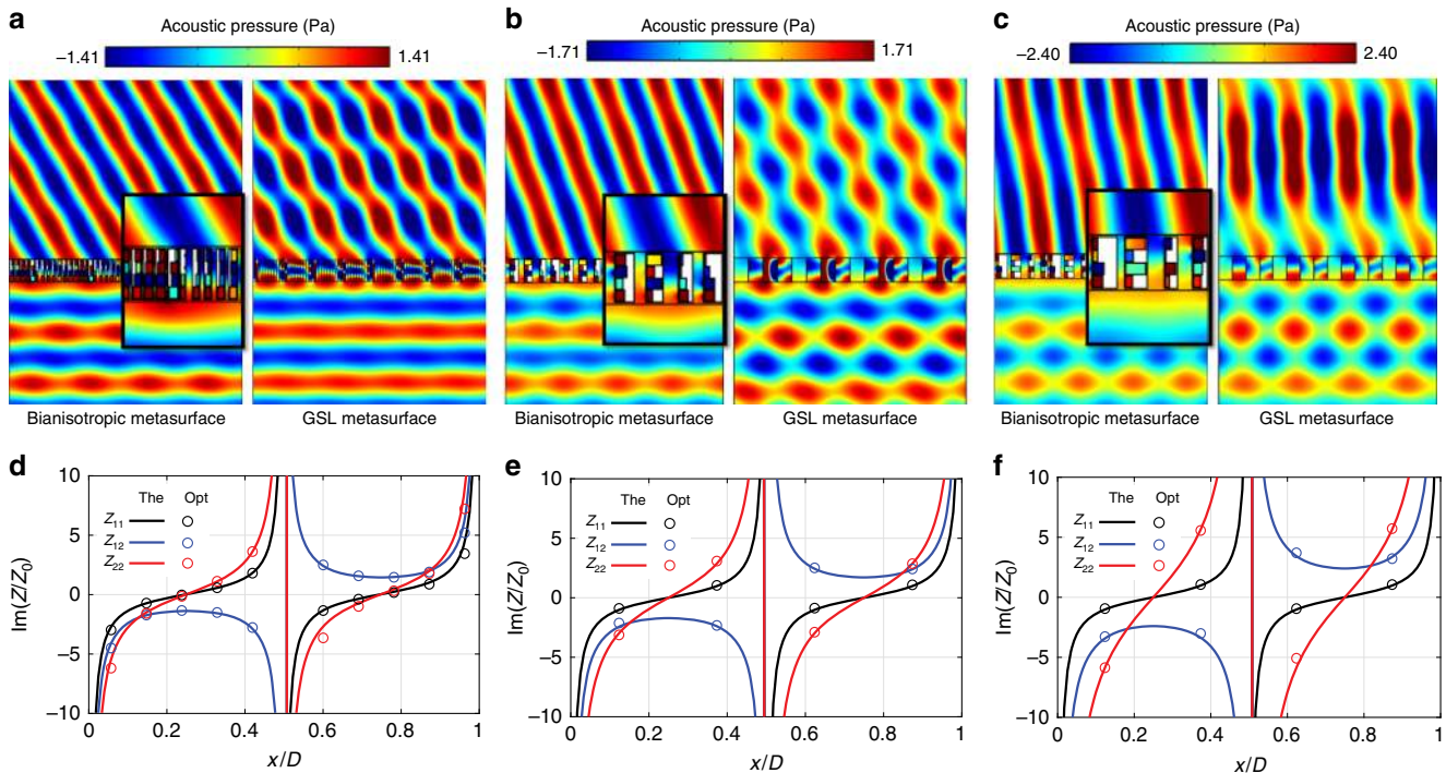
Fig. 3 Bianisotropic metasurfaces for scattering-free anomalous refraction. a–c represent the numerical simulation of the total pressure field for bianisotropic metasurfaces and GSL metasurfaces when \theta_t = 60^\circ, 70^\circ, and 80^\circ . The insets show the phase evolution inside the metasurface. d–f represent the impedance matrices profile for \theta_i = 0^\circ and \theta_t = 60^\circ, 70^\circ, and 80^\circ . Here The denotes theoretical requirements, whereas Opt denotes the impedance values achieved by structure optimization
