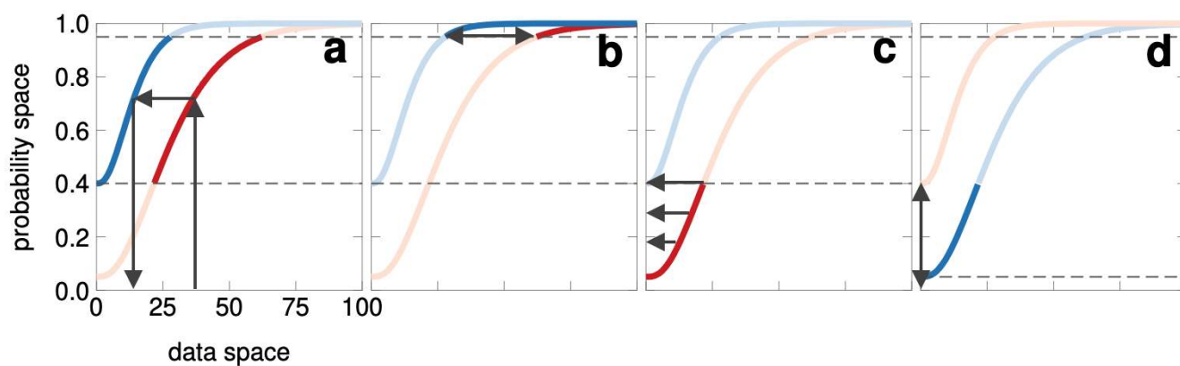
Figure A1. a) Empirical quantile mapping between model-based (red) and reference (blue) data; b) delta-approach for correcting extreme values above the maximum Weibull quantiles; c) correction of precipitation intermittency when the dry-day probability of the reference (lower dashed line) is higher; d) correction of precipitation intermittency when the dry-day probability of the reference is lower
