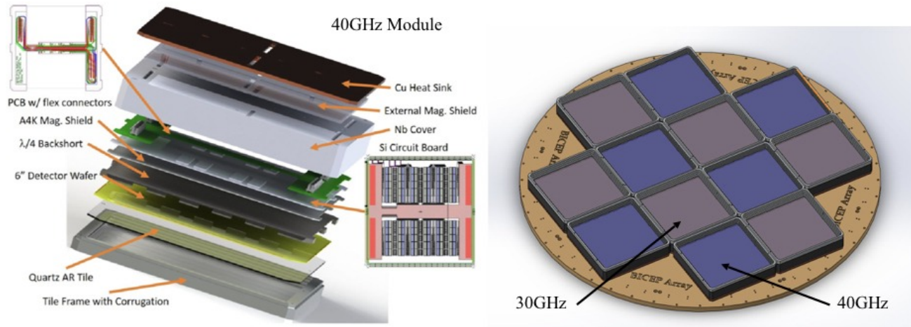
Figure 9. Left : An exploded view of the BICEP Array module. The design is based on BICEP3 but scaled to house a larger detector wafer. Right : The 30/40 GHz focal plane layout. The receiver has six 30 GHz and six 40 GHz modules laid out in a checker-board pattern.
