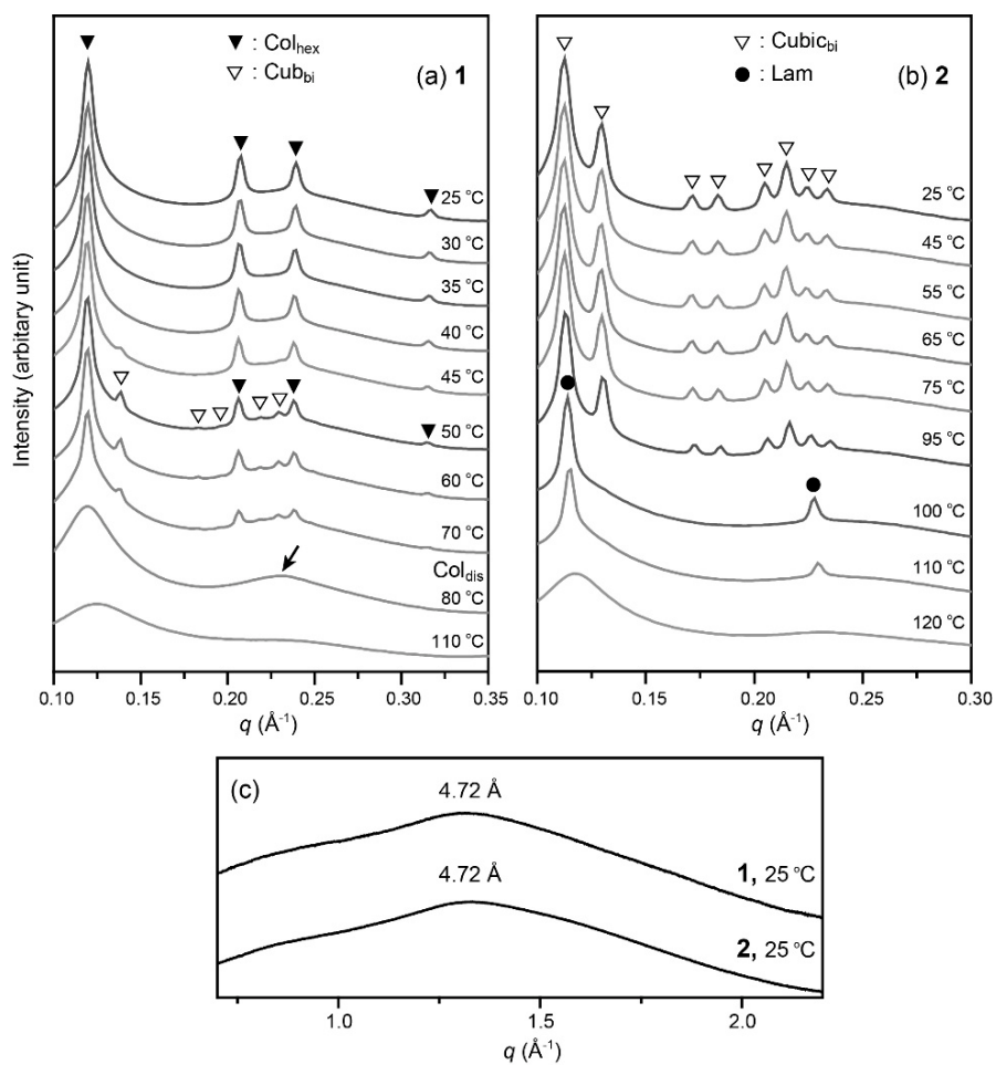
Figure 3. SAXRD data of (a) 1 and (b) 2 at various temperatures. (c) WAXRD data of 1 and 2 at RT. In (a), the arrow in the Col dis phase indicates the second reflection.
