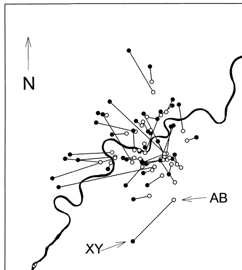
Figure 5. Actual (black circles) and mean estimated (white circles) locations of 44 places in the city of Edmonton, Alberta, Canada. The actual and estimated locations for each place are connected by a line. They were converted to pixel coordinates by hand and superimposed on a digitized map of Edmonton. The solid line running through the graph represents the actual location of the North Saskatchewan river.
