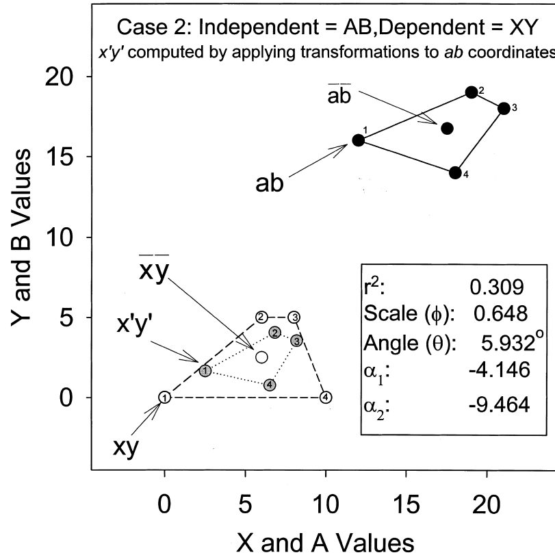
Figure 4. The toy world: The AB (cognitive map) coordinates (black dots) were the independent variable, and the XY (true map) coordinates (white dots) were the dependent variable. The gray dots represent the least squares solution. The numbers beside or inside the dots indicate corresponding coordinates.
