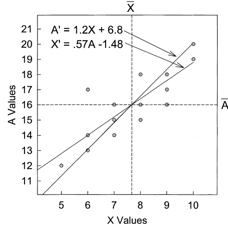
Figure 2. A set of unidimensional data (gray dots) showing the two possible regression lines: one when X is used as the independent variable and the other when A is used as the independent variable.
