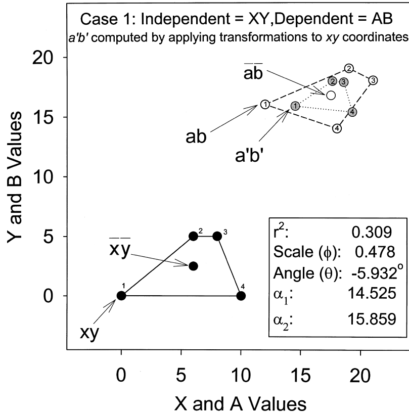
Figure 3. The toy world: The XY (true map) coordinates (black dots) were the independent variable, and the AB (cognitive map) coordinates (white dots) were the dependent variable. The gray dots represent the least squares solution. The numbers beside or inside the dots indicate corresponding coordinates.
