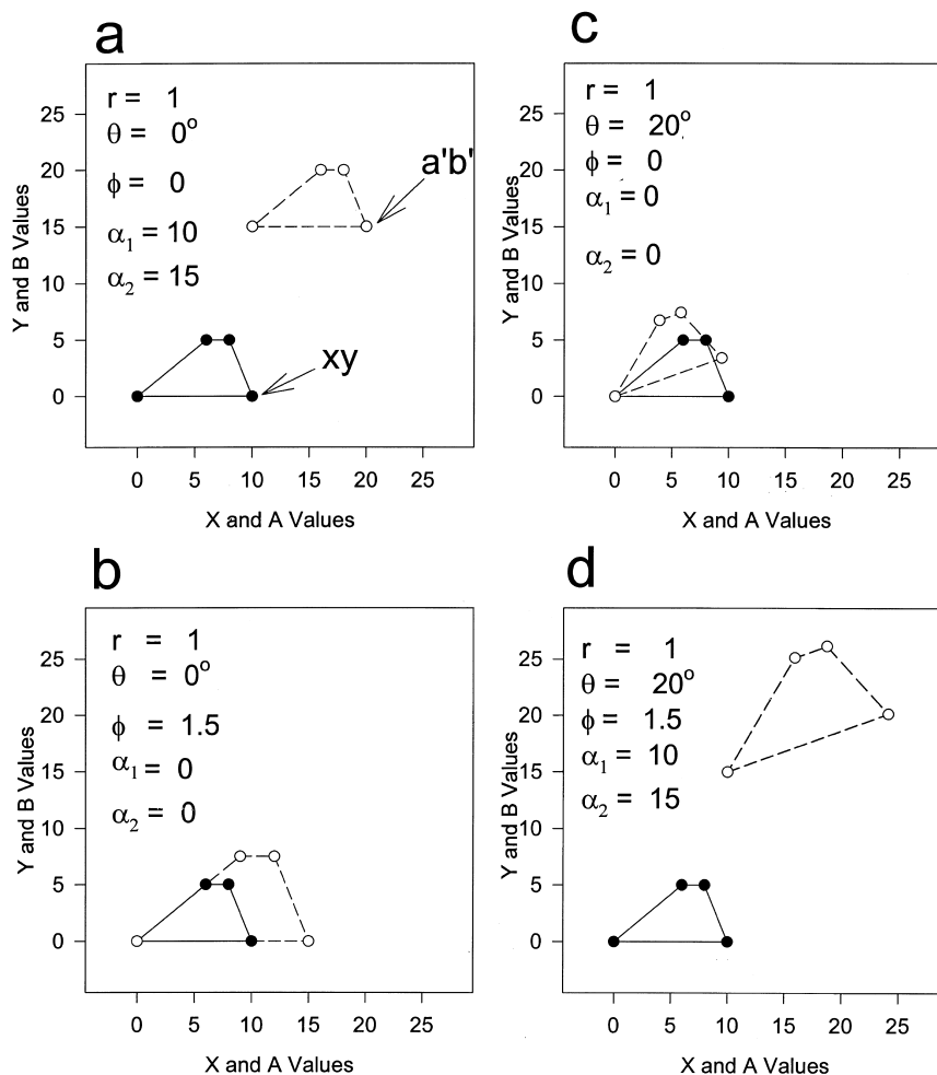
Figure 1. Bidimensional regression of a set of data in which the correlation between XY and AB is perfect. a: A simple translation of the XY coordinates. b: A scale increase. c: A rotation from the origin. d: All three transformations combined. Note that in this example, the XY coordinates serve as the independent variable in the regression.
