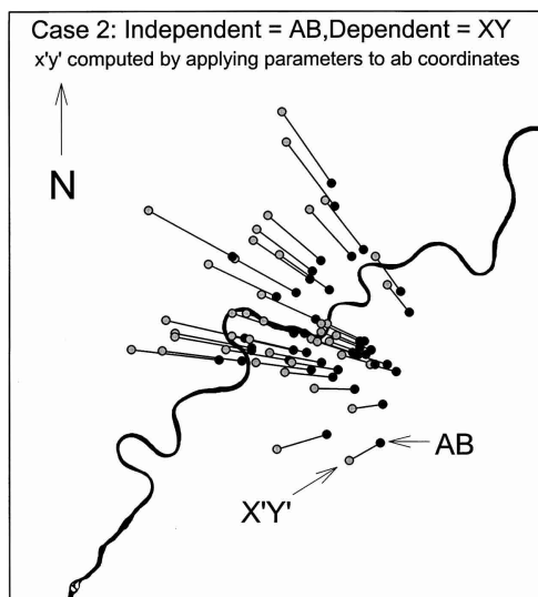
Figure 7. Mean estimated (black circles) and predicted (gray circles) locations of 44 places in the city of Edmonton, Alberta, Canada. The parameter estimates were obtained by assuming that the AB (cognitive map) coordinates were the independent variable. The estimated and predicted locations for each place are connected by a line. The estimated street and avenue locations were converted to pixel coordinates by hand, and the scale and angle transformations from Table 5, Column 3, were applied to the pixel values. The translation parameters were found by converting the mean actual and estimated street and avenue values to pixel units by hand and using the results in Equation 2.9. The final predicted values were superimposed on a digitized map of Edmonton. The solid line running through the graph represents the actual location of the North Saskatchewan river.
