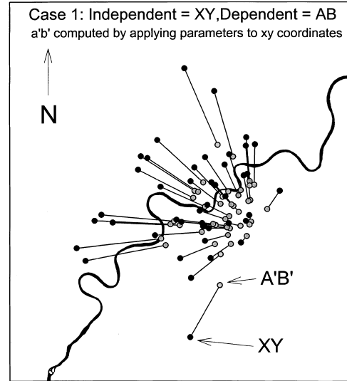
Figure 6. Actual (black circles) and predicted (gray circles) locations of 44 places in the city of Edmonton, Alberta, Canada. The parameter estimates were obtained by assuming that the XY (true map) coordinates were the independent variable. The actual and predicted locations for each place are connected by a line. The actual street and avenue locations were converted to pixel coordinates by hand, and the scale and angle transformations from Table 5, Column 1, were applied to the pixel values. The translation parameters were found by converting the mean actual and estimated street and avenue values to pixel units by hand and using the results in Equation 2.3. The final predicted values were superimposed on a digitized map of Edmonton. The solid line running through the graph represents the actual location of the North Saskatchewan river.
