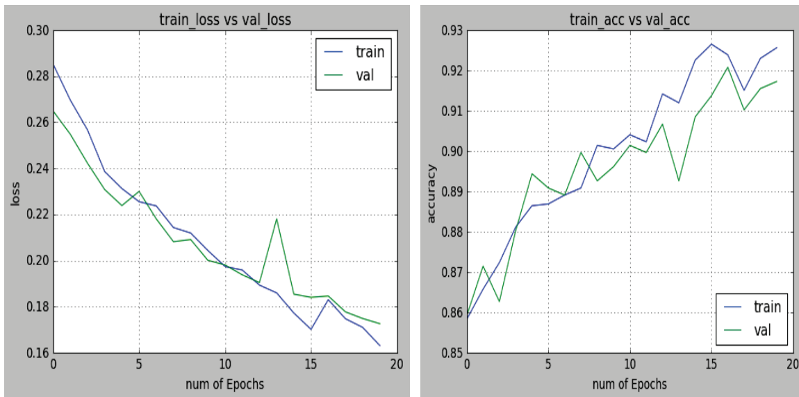
Figure 6 Accuracy and Loss for classification using GoogLeNet
