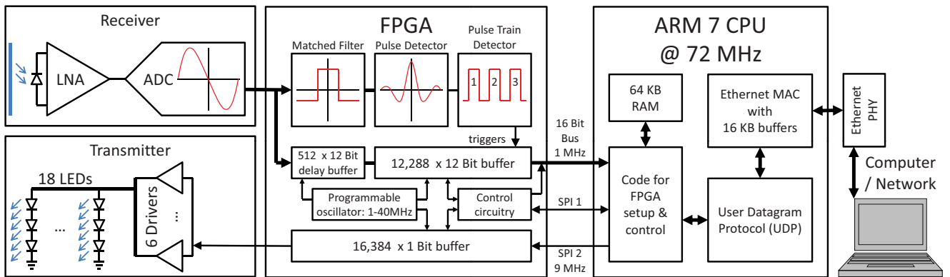
Fig. 3. Overview of the AquaOptical II hardware and software. The hardware consists of a transmitter and a receiver module, and FPGA, and a CPU. The hardware is described in detail in section III-B. The software modules are located inside the FPGA and CPU and are described in section III-C.
