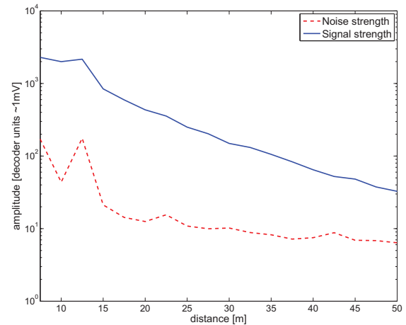
Fig. 6. Signal Strength vs Noise Strength. The x-axis indicates the transmission distance. The y-axis is logarithmic and indicates signal and noise strength in decoder units (roughly 1 mV). The blue line indicated signal strength and the red line noise levels. The beginning of the signal strength curve is capped at about 2,300 because the sensor was saturated. This is also the reason for increased noise at short distances.
