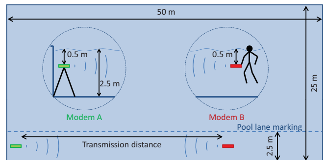
Fig. 4. Experimental Setup: Top view of the Olympic size pool (50 m x 25 m) with side views in the dotted circles. Modem A (green, left) was mounted on a tripod. Modem B (red, right) was held by a swimmer. See section IV-A for details.
