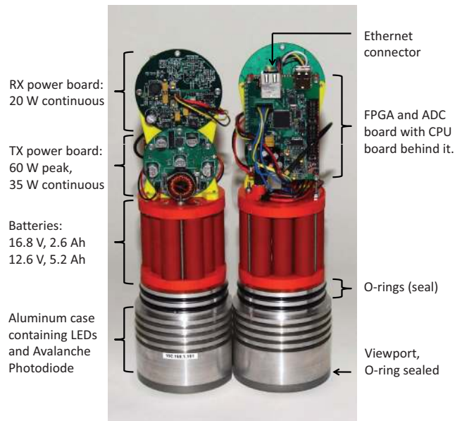
Fig. 2. Two AquaOptical II modems with the acrylic housing removed.
