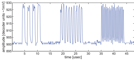
Fig. 5. Sample waveform transmitted by modem A and recorded by modem B. The x-axis shows the time in microseconds. The y-axis indicates the recorded APD output in decoder units (roughly 1 mV). The signal was sampled at 8 Mega samples per second. The width of the pulses for the three groups are, from left to right: 1 \mu sec (0.5 MHz), 500 nsec (1 MHz), 250 nsec (2 MHz).
