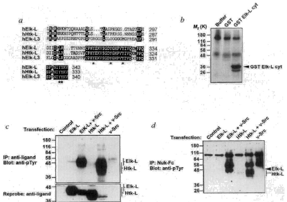
FIG. 1 Phosphorylation of transmembrane ligands by v-Src. a , Alignment of human Elk-L, Htk-L and Elk-L3 cytoplasmic domains. Black and grey boxes indicate residues conserved in all or two TM-ligands, respectively; asterisk indicates conserved tyrosines. Elk-L is also referred to as Lerk-2 [13] and Cek5-L [14], Htk-L as Lerk-5 [26] and Elf-2 [15] and Elk-L3 as NLERK-2 [29]. b , Phosphorylation of GST-hElk-L cytoplasmic-domain fusion protein (GST-Elk-L cyt) in vitro by v-Src. v-Src was immunoprecipitated from v-src-transformed Rat-2 cells and incubated with GST fusion proteins in the presence of [ \gamma - ^{32} P]ATP. c , d , Tyrosine phosphorylation of Elk-L and Htk-L upon coexpression with v-Src in Cos-1 cells. Ligands were immunoprecipitated with anti-ligand antibodies ( c ) or using Nuk-Fc as an affinity reagent ( d ), and immunoblotted with anti-phosphotyrosine antibodies. The band at approximately 100K in d represents cross-reaction of Nuk-Fc with protein A-HRP.
