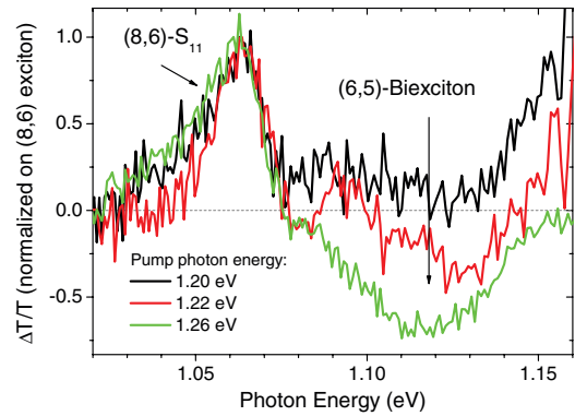
FIG. 3. (Color online) Transient spectra showing IT at 1.06 eV [(8,6)-SWCNT exciton] and IA at 1.13 eV [(6,5)-exciton-biexciton transition] after excitation at different photon energies, close to the S_{11} line. The delay between pump and probe pulses is fixed at 700 fs. The spectra have been normalized to the exciton signal for ease of comparison.
