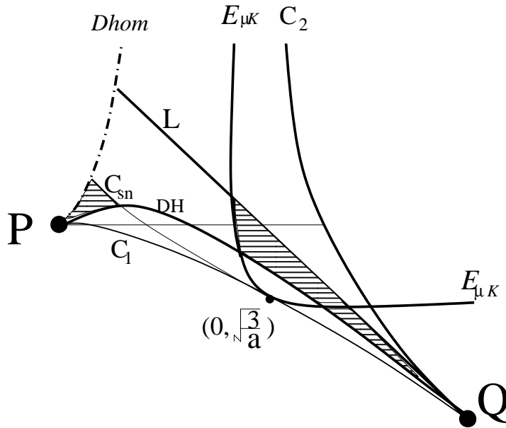
FIG. 6.3. In the shaded subregion of V_{sn} below C_{sn} , the saddle-node bifurcation of limit cycles occurs after the transcritical bifurcation involving E_\mu and E_K . In the shaded subregion of V_{sn} to the right of E_{\mu K} , the saddle-node bifurcation of limit cycles occurs before the transcritical bifurcation.
