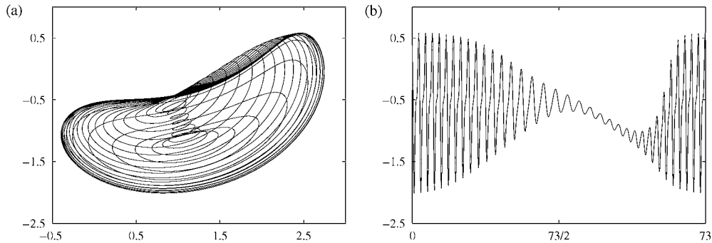
Figure 23. (a) Projection on the (y, z) plane of a limit cycle corresponding to a period-one phase-locked circle for parameter values (F, G) = (9.3, 3.0472169822) inside \mathcal{A}_{35} . (b) Same as (a), projection on the (t, z) plane.
