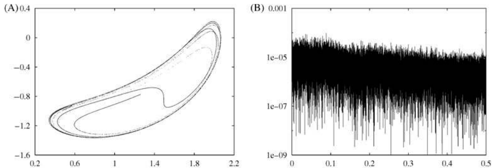
Figure 9. (A) Projection on (y, z) of the Shil'nikov-like strange \mathcal{P} -attractor \mathbb{S}_1 , occurring at (F, G) = (7, 1.7545) . (B) Power spectrum of \mathbb{S}_1 .
