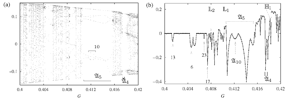
Figure 41. (a) Projection on the y-axis of sequences of \mathcal{P} -attractions as a function of G , for F = 1.25 fixed. The last 100 points of each iteration loop are plotted, the step in G is 10^{-4} . See text for explanation. (b) Maximal Lyapunov exponent on the attractors in (a).
