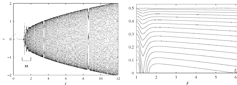
Figure 25. Left: projections on the y-axis of \mathcal{P} -attractors as a function of F for G = 0.2 fixed. F is increased with a step of 0.02. The last 100 points of each loop are plotted. Interval M is enlarged in figure 26. Right: rotation number (modulo 1/2, see appendix A.3) as a function of F . Each curve corresponds to a fixed value of G : G = 0.36 for the lowest and G = 0.08 for the upmost. Between two curves, G differs of 0.02.
