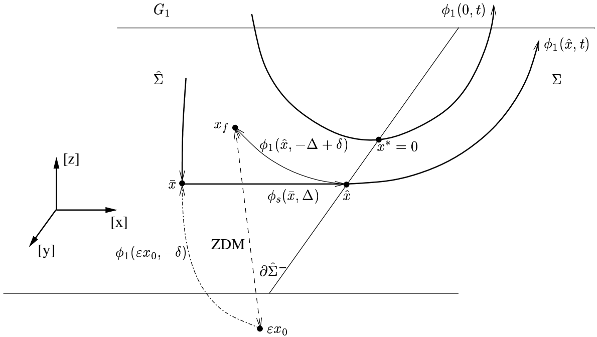
Figure 5: Schematic representation of constructing the ZDM for the case of grazing sliding bifurcation
