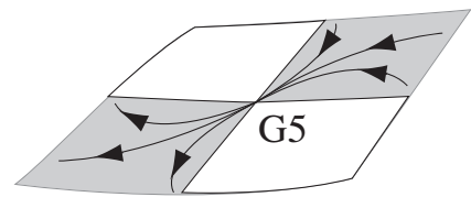
Figure 10: Generic dynamics in a piecewise smooth system: G5 consists of an open region of sliding segments that hit a two-fold. Sliding/escaping regions are shaded, crossing regions are unshaded.
