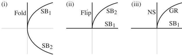
Figure 23: Partial unfolding of the codimension-two sliding bifurcations of nonhyperbolic limit cycles. (i): sliding bifurcation + fold; SB_1 and SB_2 are sliding bifurcations of the two cycles involved in the fold bifurcation. (ii): sliding bifurcation + flip; SB_1 and SB_2 are the sliding bifurcations of the period-one and period-two cycle respectively. (iii) sliding bifurcation + Neimark-Sacker; SB_1 is the sliding bifurcation of the cycle, NS is the Neimark-Sacker, and GR is a grazing bifurcation of the torus. Bifurcation curves near any of these codimension-two points must be arranged as in one of the three portraits. However, the presence of other bifurcation curves, and the dynamics across the curves, depend on the type of sliding bifurcation, and the complete unfoldings are still unknown.
