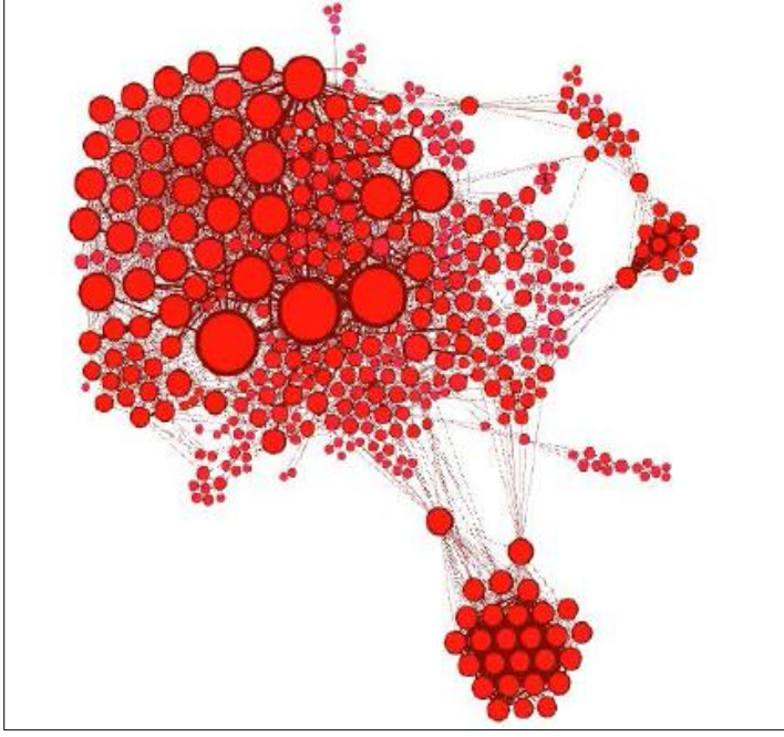
Figure 3: Force Atlas layout of 233 connected nodes
