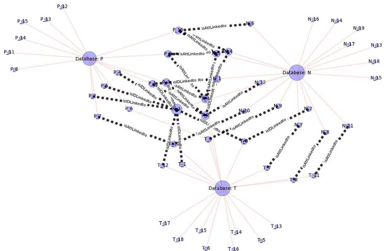
Fig. 4. SEEKER generates link hypotheses between potential field elements based on the match by the field name, data type and the histogram of a random sample of data compared against data sources. (Colors are visible in the online version of the article; http://dx.doi.org/10.3233/ISU-130712 .)
