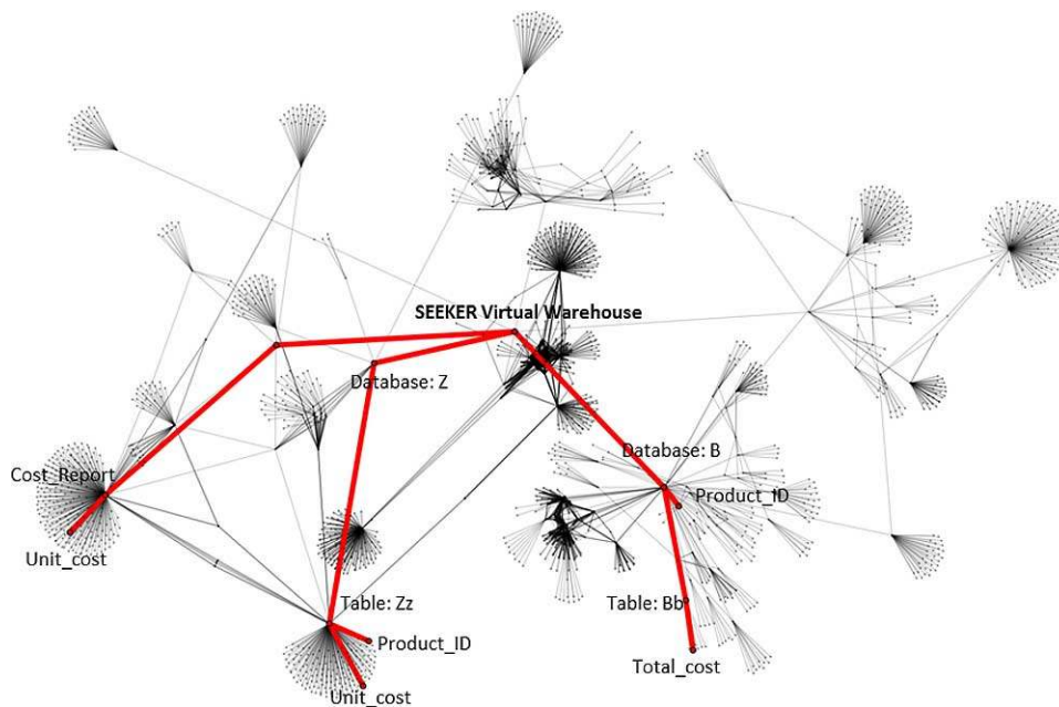
Fig. 3. Example of how SEEKER helps construct queries by showing the access path and join path while querying across data-sources. (Colors are visible in the online version of the article; http://dx.doi.org/10.3233/ISU-130712 .)
