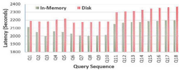
FIGURE 13. Mean latency per query for 1 million smart meters across 1-Node.
