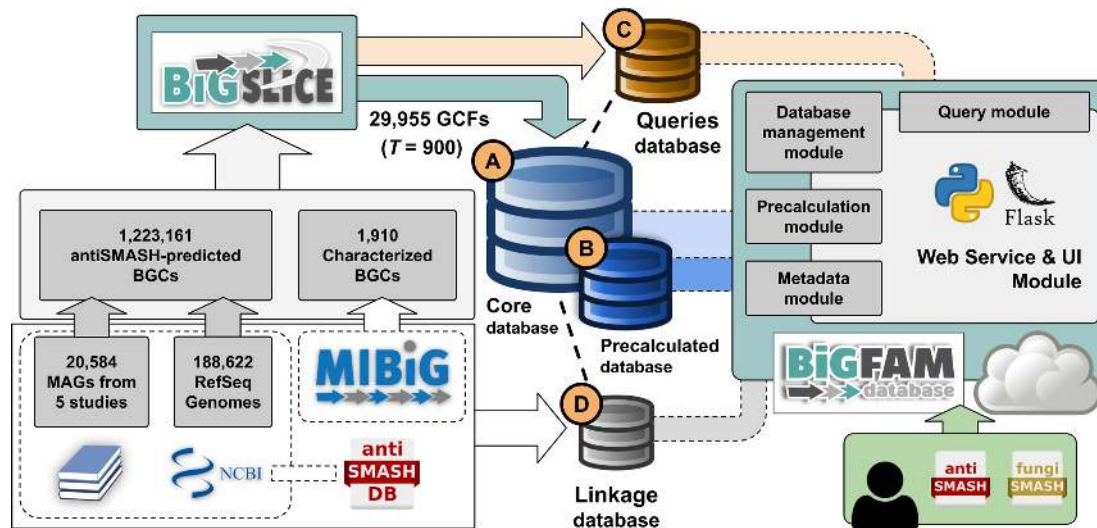
Figure 2. Workflow schema of BiG-FAM's architecture. Starting from a collection of ~1.2 million BGCs, BiG-SLiCE was used to perform a clustering analysis (with threshold parameter T = 900 ), resulting in (A) 29,955 GCFs stored in an SQLite3 database file. This file is used as the 'Core database' for BiG-FAM. To support BiG-FAM's extensive functionalities, three related database files were created, each managed by a specific module in the software package. (B) The 'Precalculated database' summarizes complex SQL operations (i.e., calculation of taxonomy counts per GCF) to speed up page loads (detailed schema and procedures can be accessed from the 'precalculation' module in BiG-FAM's source code). (C) The 'Queries database' stores information related to user-submitted BGC queries, such as processed features from antiSMASH BGCs and the corresponding list of best-matched GCFs identified using BiG-SLiCE. (D) Finally, the 'Linkage database' keeps tabs on the cross-links to external databases (i.e. MIBiG and antiSMASH-DB), storing information such as the accession number of each linked BGC, which can be used to generate the correct URL addresses pointing to the correct entry within the specific database. These modules and databases were used to serve an online database written in Python using the Flask programming library.
