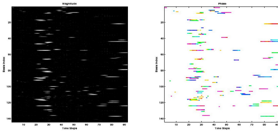
Figure 6. Coding of a 100-frame image sequence in terms of magnitude (left) and phase (right). Vertical axis is coefficient index and horizontal axis is time. Phase is displayed for only those points in time when the corresponding amplitude is significant.
