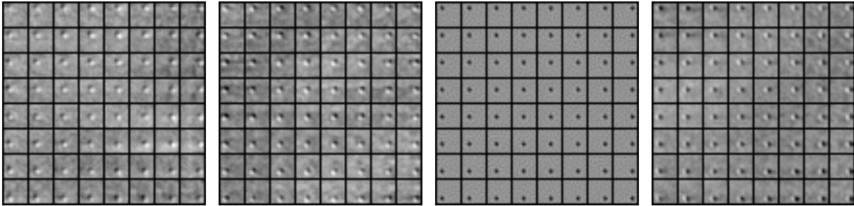
Figure 4. Four of the remapping bases, \Psi_k(\mathbf{x}, \mathbf{x}') , learned from the transformations contained in natural image sequences. Each basis function shows how a pixel in one frame is mapped into the next frame—i.e., each patch within a basis function corresponds to a pixel within the originating frame (ordered according to its position in the frame), and the values within the patch denote how it is weighted into the next frame. For example, the identity function (third from left) simply maps each pixel into itself.
