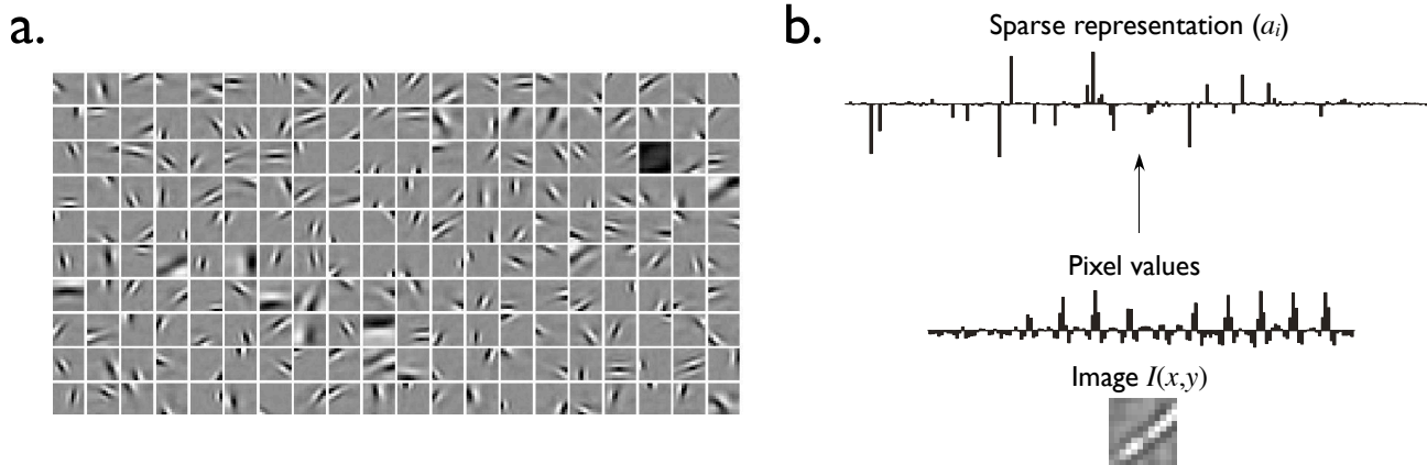
Figure 1. a. Features learned from sparse coding of natural images. Each patch shows a different basis function, \phi_i , and together the entire set of functions can be used to describe a 12 \times 12 pixel image patch. b. An example image patch (bottom) and its representation in terms of the coefficients, a_i , shown as a bar chart (top).
