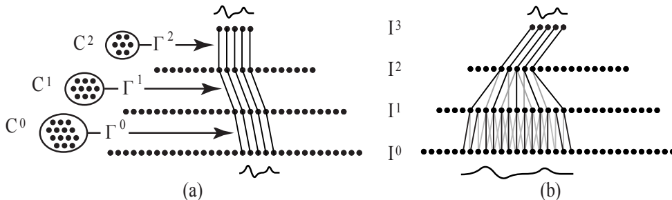
Figure 2. Hierarchical remapping circuit composed of three bilinear stages. The units at each level l , I_i^l , compute their values from a weighted sum of units in the level below, I_i^l = \sum_j W_{ij}^l I_j^{l-1} . The weights in turn are dynamically modulated by the control neurons, C , via W_{ij}^l = \sum_k \Gamma_{ijk}^l C_k^l . Shown in a. and b. are two different settings of the weights which allow different instantiations of the same pattern to be remapped into a common pattern at higher levels.
