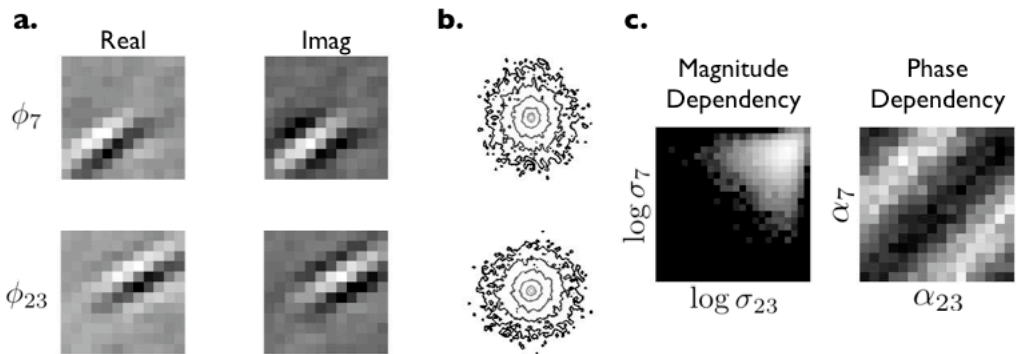
Figure 5. a. Each row shows a different complex basis function pair learned in the shiftable basis function model. The real part of each function is shown at left, and the corresponding imaginary part is shown at right. b. Joint histogram of the real and imaginary coefficients, u_i, v_i for each complex pair. c. Joint histograms of log-amplitude (left) and phase (right) for the pair of complex basis functions shown at left.
