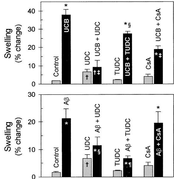
Fig. 4. Percent change in mitochondrial swelling following incubation of isolated mitochondria with UCB and A \beta peptide. Mitochondria were isolated and incubated with either no addition (control), 4.3 \mu M unconjugated bilirubin (UCB), 125 \mu M amyloid- \beta (A \beta ) peptide (25–35), or a combination of toxic agent plus 500 \mu M ursodeoxycholate (UDC), 500 \mu M tauroursodeoxycholate (TUDC) or 5 \mu M cyclosporine A (CsA) in respiration buffer as described in “Materials and Methods.” At 5 min, the apoptotic agent was added and the percent change in mitochondrial swelling from 5 to 10 min was determined by monitoring the absorbance at 540 nm. In the coinubation experiments, mitochondria were pretreated with UDC, TUDC, or CsA for 5 min. The results are means \pm standard error of the mean (SEM) of at least three separate experiments. † p < 0.05 , * p < 0.001 from control; § p < 0.05 , ¶ p < 0.01 , ‡ p < 0.001 from toxic stimuli alone.
