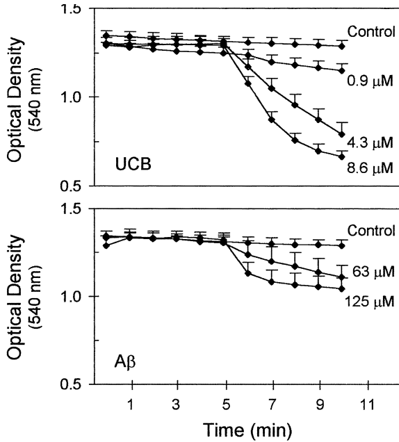
Fig. 3. Dose-response of isolated mitochondria to UCB- and A \beta peptide-induced swelling. Mitochondria were isolated and incubated with either no addition (control), unconjugated bilirubin (UCB; 0.9, 4.3, and 8.6 \mu M), or amyloid- \beta (A \beta ) peptide (25–35) (63 and 125 \mu M) in respiration buffer as described in “Materials and Methods.” At 5 min, the apoptotic agent was added and the decrease in absorbance at 540 nm was monitored for an additional 5 min-period. The results are means \pm standard error of the mean (SEM) of at least three separate experiments.
