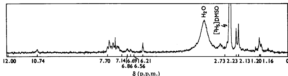
Fig. 7. N.m.r. spectrum of azo pigment S_5 in [^2H_6] dimethyl sulphoxide ( [^2H_6] DMSO). The spectrum was recorded from a saturated solution (approx. 0.01 M). Chemical shifts are given in p.p.m. relative to tetramethylsilane = 0 (internal standard). Assignments are presented in the text.
