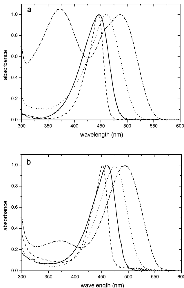
Fig. 2 Normalized UV/Vis absorption spectra of PYP hybrids: (a) WT PYP apoprotein, (b) E46Q PYP apoprotein; pCA (—), locked (---), fer (···), sin (-·-). Spectra of protein reconstituted with different chromophores were taken in the dark, in 50 mM phosphate buffer, pH 7.5.
