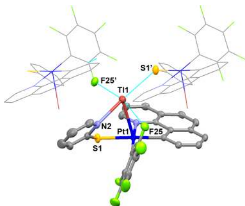
Figure 2. Molecular structure of [\{Pt(C_6F_5)(bzq)\}Tl(Spy)] ( 2-y ) showing the environment of the Tl I center. Asymmetric unit and selected atoms shown as 50% probability thermal ellipsoids.
