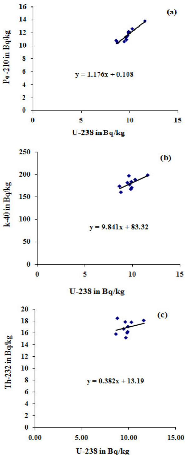
Figure 2. Relation between the activity concentrations of different radionuclides in Eleaocarpus oblangus samples.
