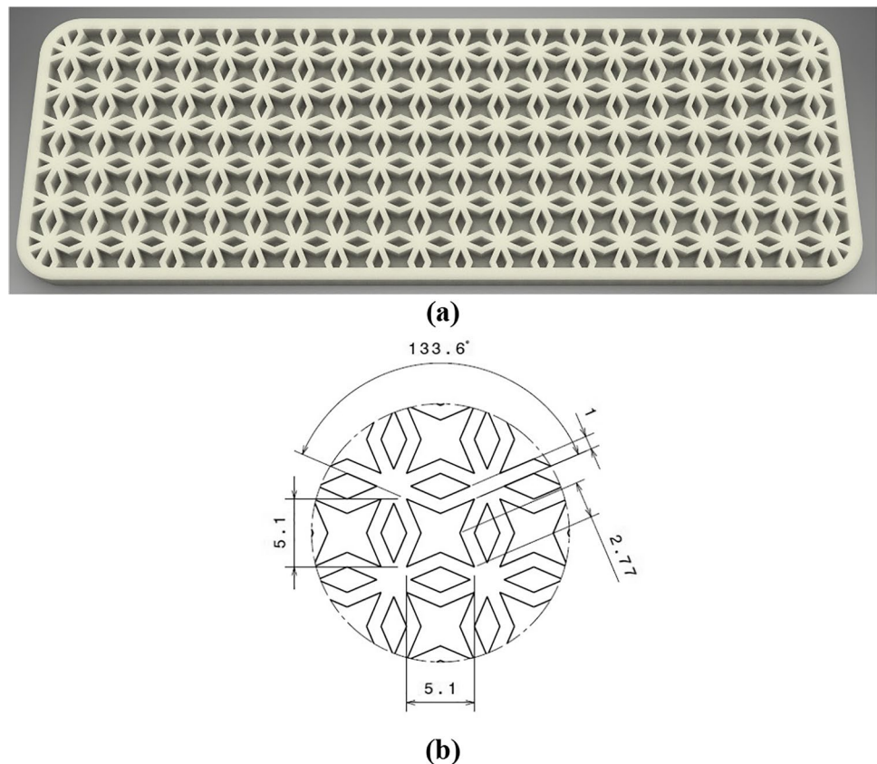
Fig. 15 a Star-shaped lattice core structure; b dimensions of the star-shaped unit cell.
