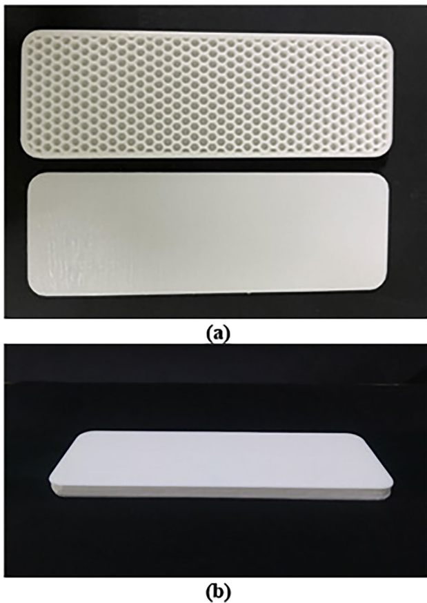
Fig. 5 a Two 3D-printed parts of the small-scale deck; b two parts assembled with adhesive
