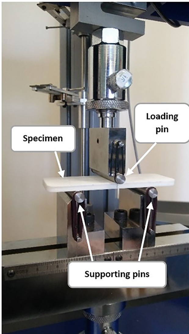
Fig. 7 The scale model deck with a honeycomb structure core under the three-point bending test.
