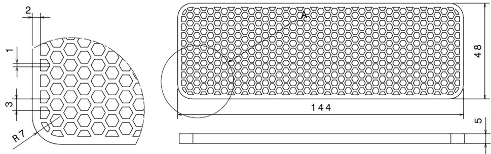
Fig. 3 2D definition of the bio-inspired honeycomb lattice structure (dimensions are in mm)
