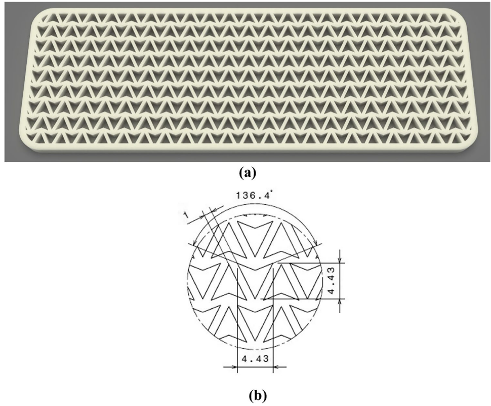
Fig. 16 a Arrowhead lattice core structure; b dimensions of the arrowhead unit cell
