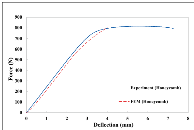
Fig. 10 Comparison between numerical and experimental load-deflection responses of the honeycomb scale model of decks under the three-point bending test.
