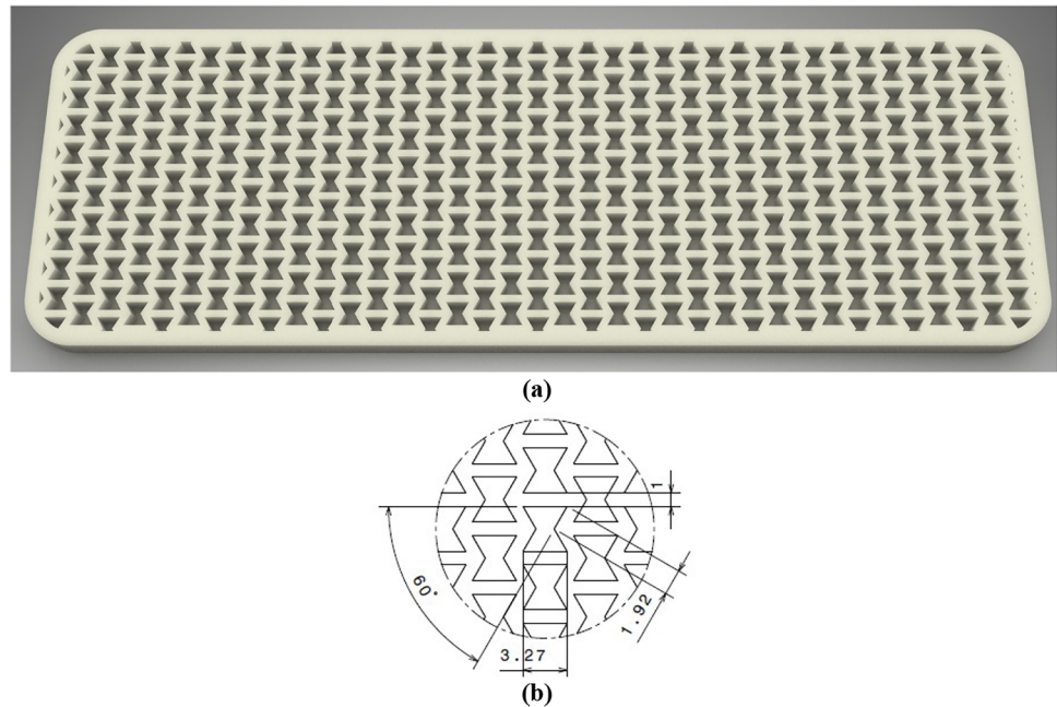
Fig. 11 a Re-entrant lattice core structure; b 2D definition with dimensions of the re-entrant unit cell
