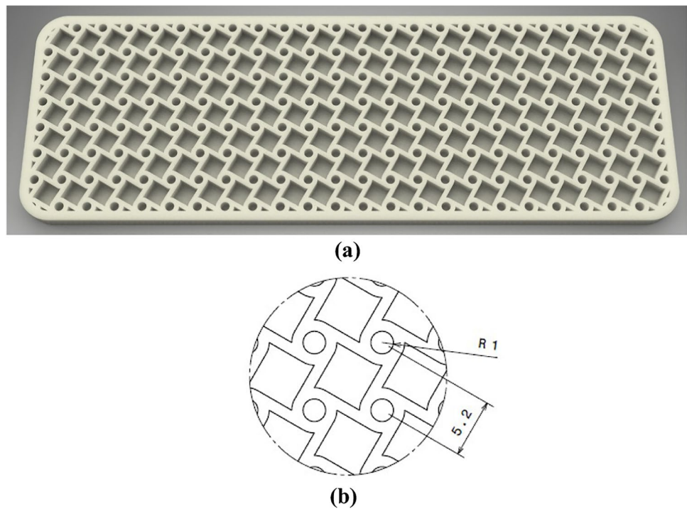
Fig. 13 a Tetrachiral lattice core structure; b dimensions of the tetrachiral unit cell
