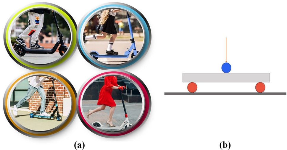
Fig. 6 a The most common situations of the rider's feet: when the rider's foot is placed in the middle of the deck, the maximum force is exerted, b three-point bending schematic.
