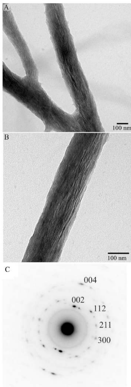
Figure 5. TEM images of mineralized collagen fibrils for 16 hours at low (A) and intermediate (B) magnifications and (C) the diffraction pattern taken from area in (B).
