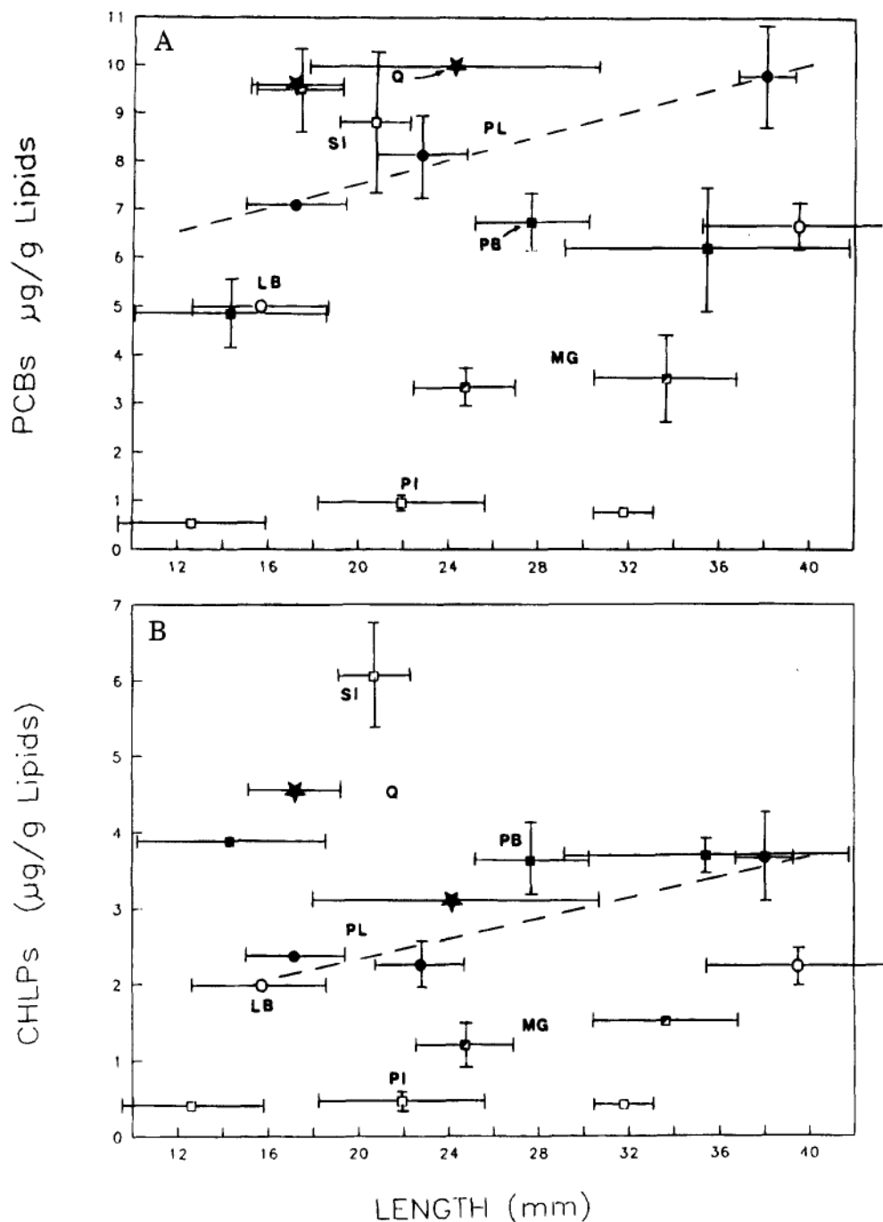
FIGURE 4. Total concentrations of PCBs (A) and chlorinated pesticides (B) in Asiatic clams versus clam length.
