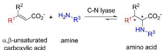
Scheme 1. Direct hydroamination of \alpha,\beta -unsaturated carboxylic acids catalyzed by a C–N lyase with enantiocontrol to synthesize optically pure \alpha -amino acids.
