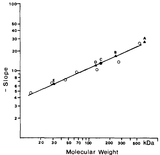
Fig. 3. Standard curve of molecular weight by minus slope in Fig. 2. Open circle (○): standard proteins, closed circle (●): A-antigen (=band C in disc-PAGE), closed triangle (▲): component proteins in CF.
