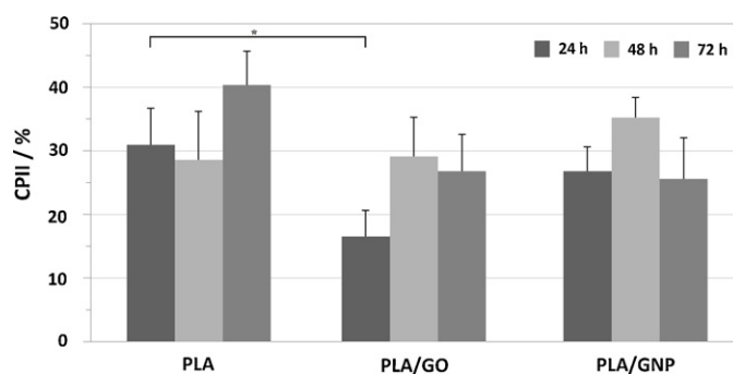
Fig. 7. Cell proliferation inhibition index for mouse embryo fibroblasts, cultured on PLA, PLA/GO and PLA/GNP films. Results are presented as mean and error bars represent SD. *Significantly different ( p < 0.05 ).
