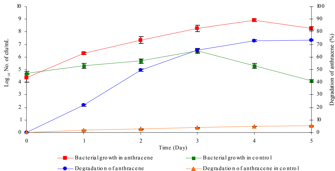
Fig. 9. Degradation of anthracene (3 mg/L) by halotolerant bacterial consortium at 60g/L of NaCl concentration in the presence of yeast extract (0.2 g/L)
