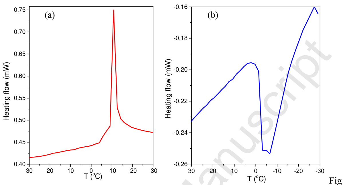
Figure 15): The DSC (a) cooling and (b) heating curves for obtained biodiesel
