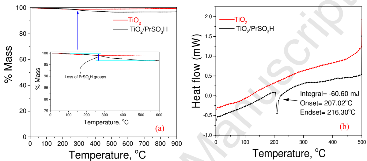
Figure (10): TGA (a) and DSC (b) profiles for \text{TiO}_2 and \text{TiO}_2/\text{PrSO}_3\text{H} nano-catalysts
