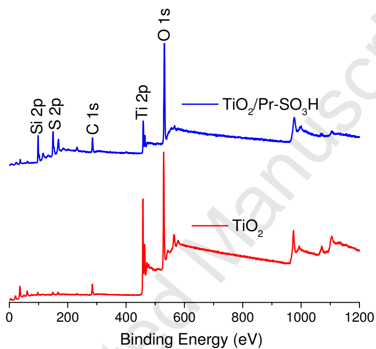
Figure (8): XPS survey scan of \text{TiO}_2 -NPs and synthesised \text{TiO}_2/\text{PrSO}_3\text{H} nano-catalysts
