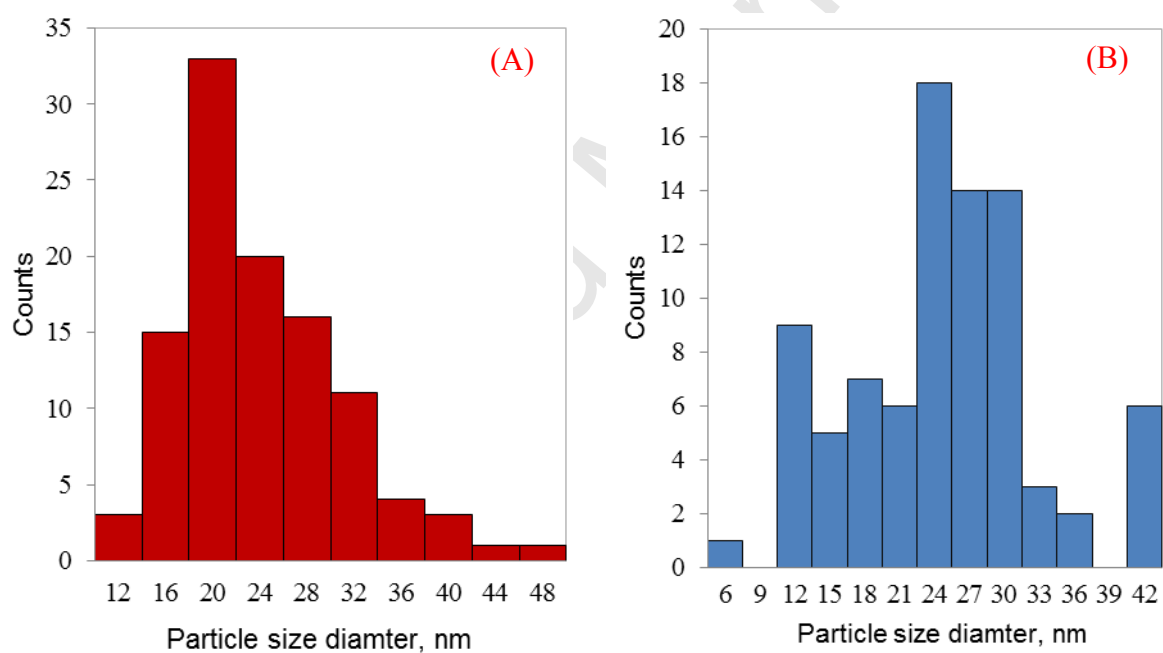
Figure (4): Particle size distributions for (a) \text{TiO}_2 and (b) \text{TiO}_2/\text{PrSO}_3\text{H} nano-catalysts
