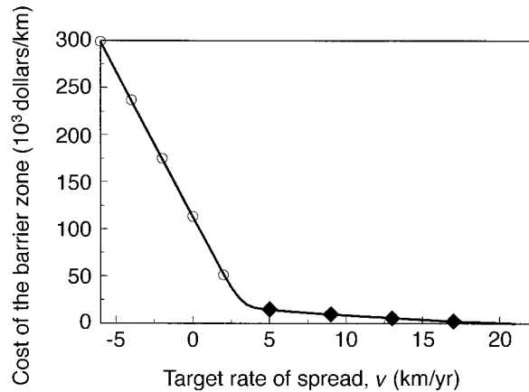
FIG. 7. Expected cost of the barrier zone per 1 km length for various target rates of gypsy moth spread. The line is fitted from Eq. 14; ◆ represents the model of Sharov et al. (1998); ○ represents Eq. 13.
