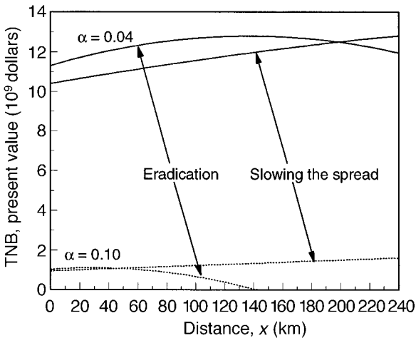
FIG. 9. Total net economic benefits (TNB) from either slowing the spread or doing a one-step eradication of a circular gypsy moth population of radius x ; \alpha is the discount rate.
