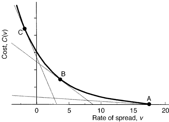
FIG. 3. Cost of the barrier zone per unit length for varying target rates of population spread. The optimal target rate of spread of the population expanding along an infinite strip is equal to the point where the tangent of function C(v) is equal to -D/\alpha . Depending on the slope, the optimal strategy may be no management (A), slowing the spread (B), or eradication (C).
