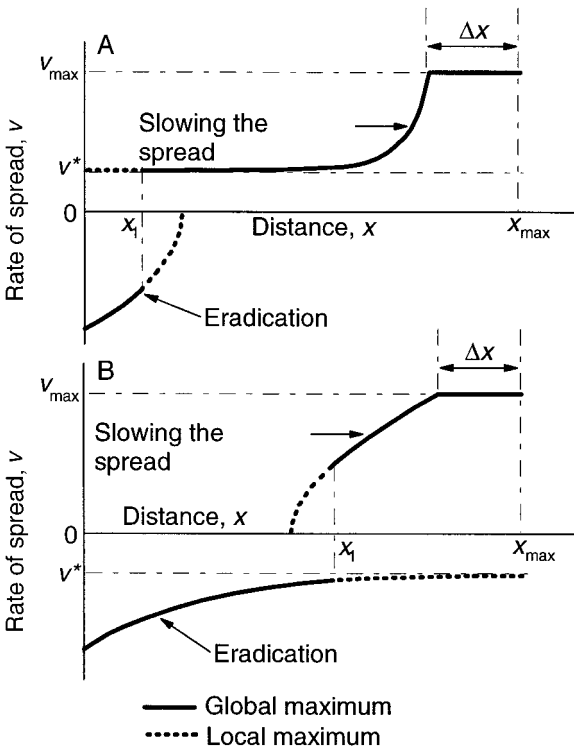
FIG. 5. Optimal management of the rate of population spread, v , in a rectangular area; v^* is the solution of Eq. 6. v_{\max} is the rate of unmanaged spread, and \Delta x is the distance defined by the boundary condition (Eq. B.6). Graphs (A) and (B) correspond to v^* > 0 and v^* < 0 , respectively. The global maximum corresponds to a strategy that yields the highest net benefits (benefits are not shown in this graph). The local maximum corresponds to a strategy yielding net benefits that are higher than for any small variation of this strategy, but the local maximum is lower than the global maximum.
