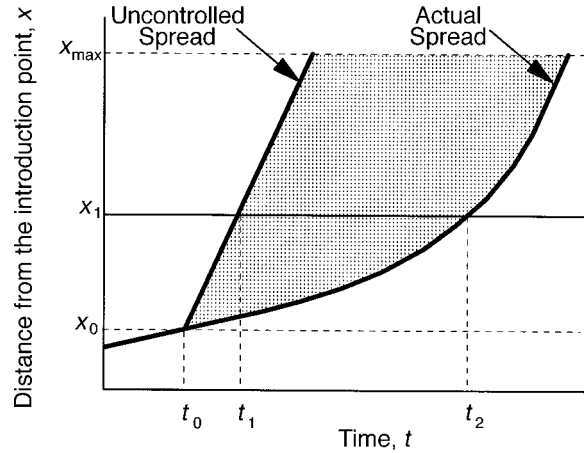
FIG. 4. Dynamics of actual (managed) and uncontrolled population spread. The shaded area is the spatiotemporal region where benefits from slowing population spread are gained; x_{\max} is the most distant point in the uninfested area.
