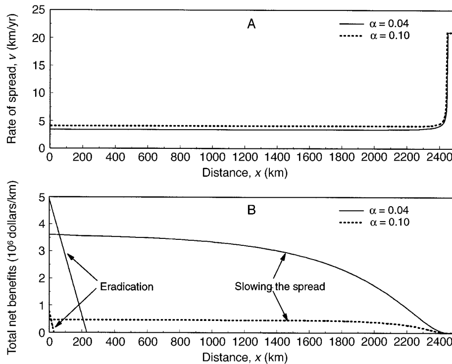
FIG. 8. (A) The optimal target rate of gypsy moth spread, and (B) economic benefits (present value) per 1 km length of the population front that result from either slowing population spread or one-step eradication, predicted by the model that assumes population spread in a rectangular potential range starting at varying distances, x , from one side; \alpha is the discount rate.
